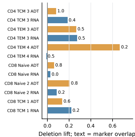
f Attribution faithfulness
