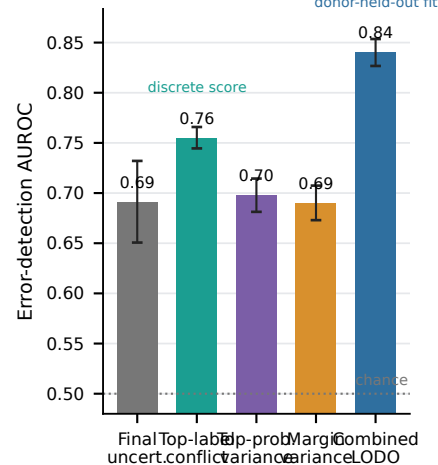
c Audit-score error detection
