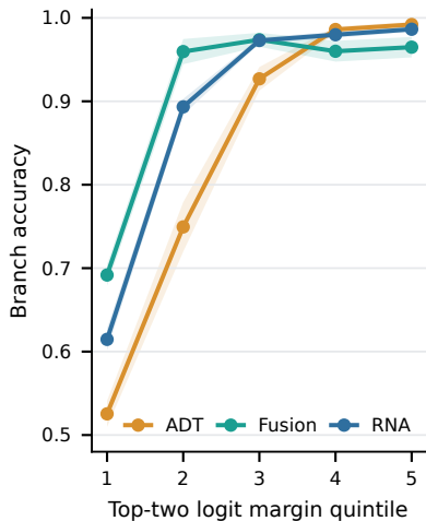
d Margin-correctness audit
