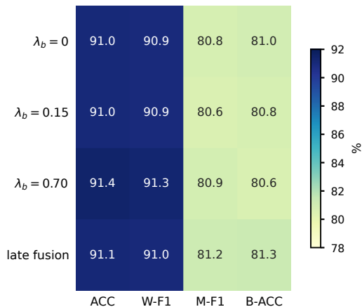
b Branch-loss sensitivity
