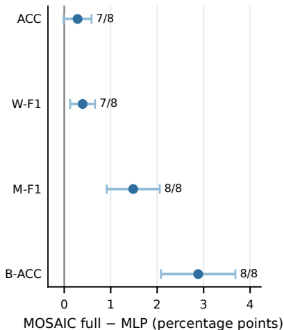
a Primary donor effect
