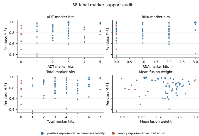
Figure 3 58-label marker-support audit. Each point is one PBMC L3 label; point size is held-out test support and color indicates whether a non-empty representative ADT marker list is fully present. Panels show per-class M-F1 against ADT hits, RNA hits, total hits and mean fusion weight. The descriptive Spearman associations are near zero, so panel availability and top-20 attribution use are not interchangeable evidence types.
