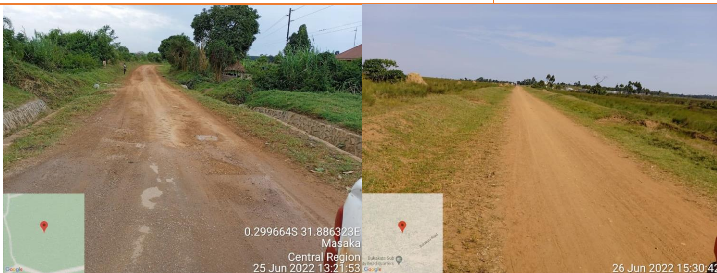
Photograph 2-10: Potholes and poor formation level along Mukoko - Birinzi - Ssunga road
