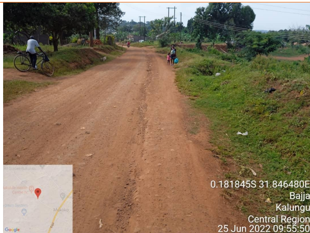
Photograph 2-2: Rutting along Bukulula - Kalungu road.
