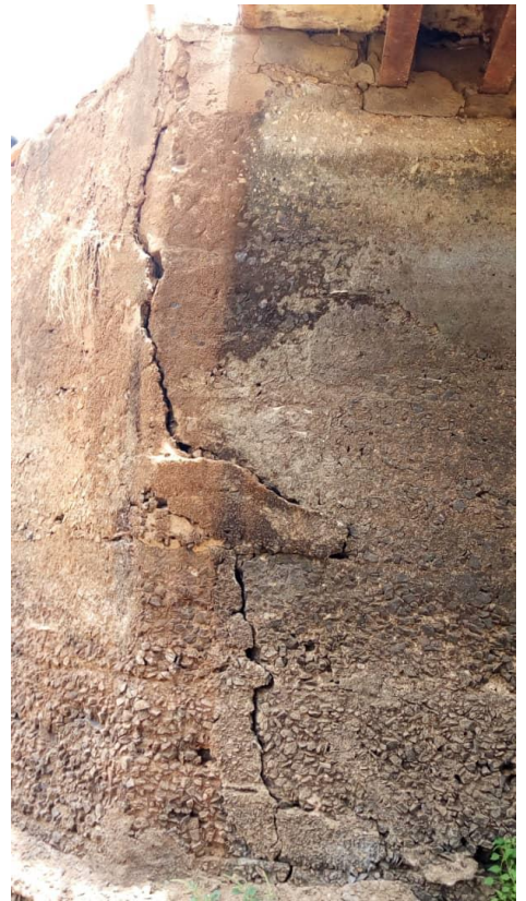
Omposo Bridge (B333) along Moyo – Obongi (C722_Link01) road in very poor condition
