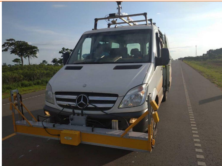
Photograph 1-15: ROMDAS surveys on the newly upgraded pavement along Tirinyi - Pallisa - Kumi road.
