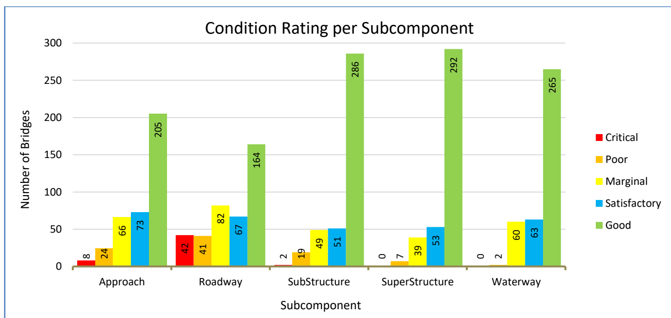
Figure 6-2: Condition rating of bridges per subcomponent
