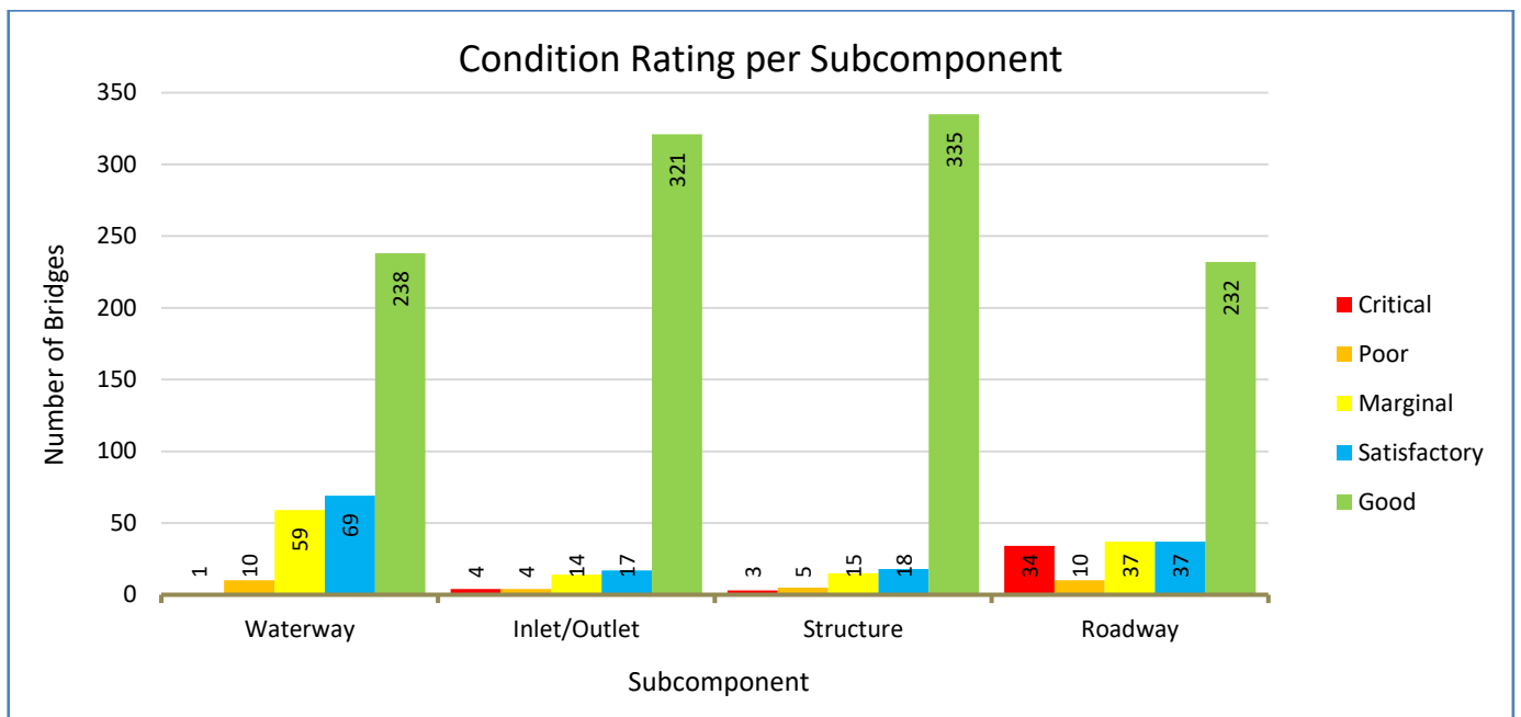
Figure 6-4: Condition rating of major culverts per subcomponent
