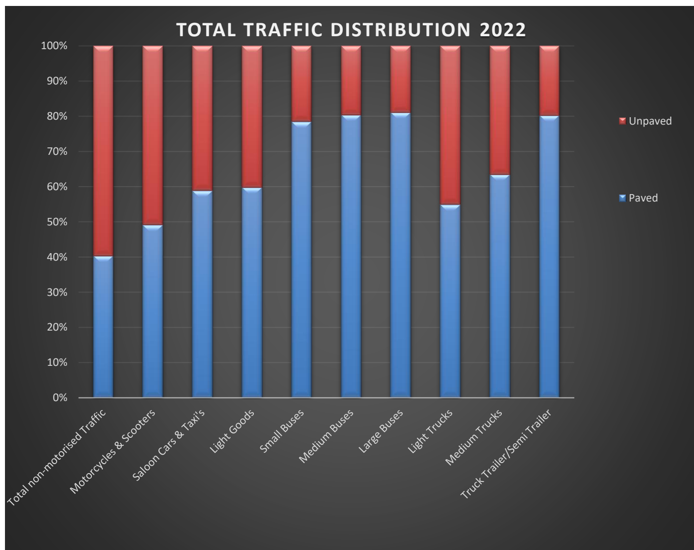
Figure 3-2: Total Traffic distribution for each surface type per Vehicle Type, 2022
