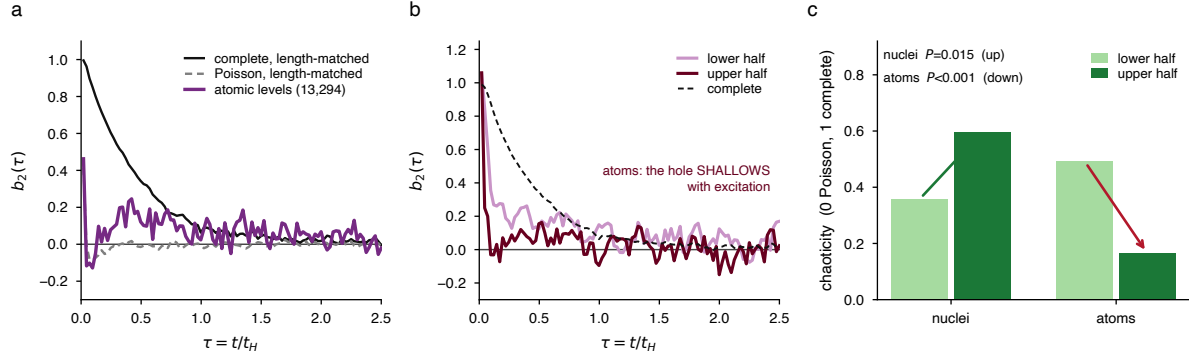
Figure 6: Two measured spectra give the same completeness estimate for opposite reasons. a , Atomic form factor against length-matched complete and Poisson references. b , The same sequences split at their own median energy. c , Chaoticity of the lower and upper halves for both datasets. In nuclei the hole deepens with excitation, which is chaos setting in; in atoms it shallows, which is detection efficiency falling. The estimator returns \phi \approx 0.30 in both cases.
