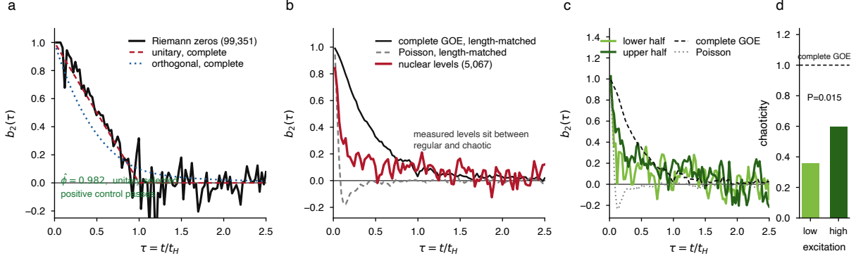
Figure 5: Real spectra: a control that is complete, and measured levels that are not incomplete but not yet chaotic. a , Riemann zeros, complete by construction. The pipeline selects unitary symmetry and returns \hat{\phi} = 0.982 . b , Measured nuclear levels against length-matched complete and Poisson references. c , The same sequences split at their own median energy. d , Chaoticity, scaled so Poisson is 0 and a complete chaotic spectrum is 1. The hole deepens with excitation energy, which is chaos setting in rather than levels going missing.
