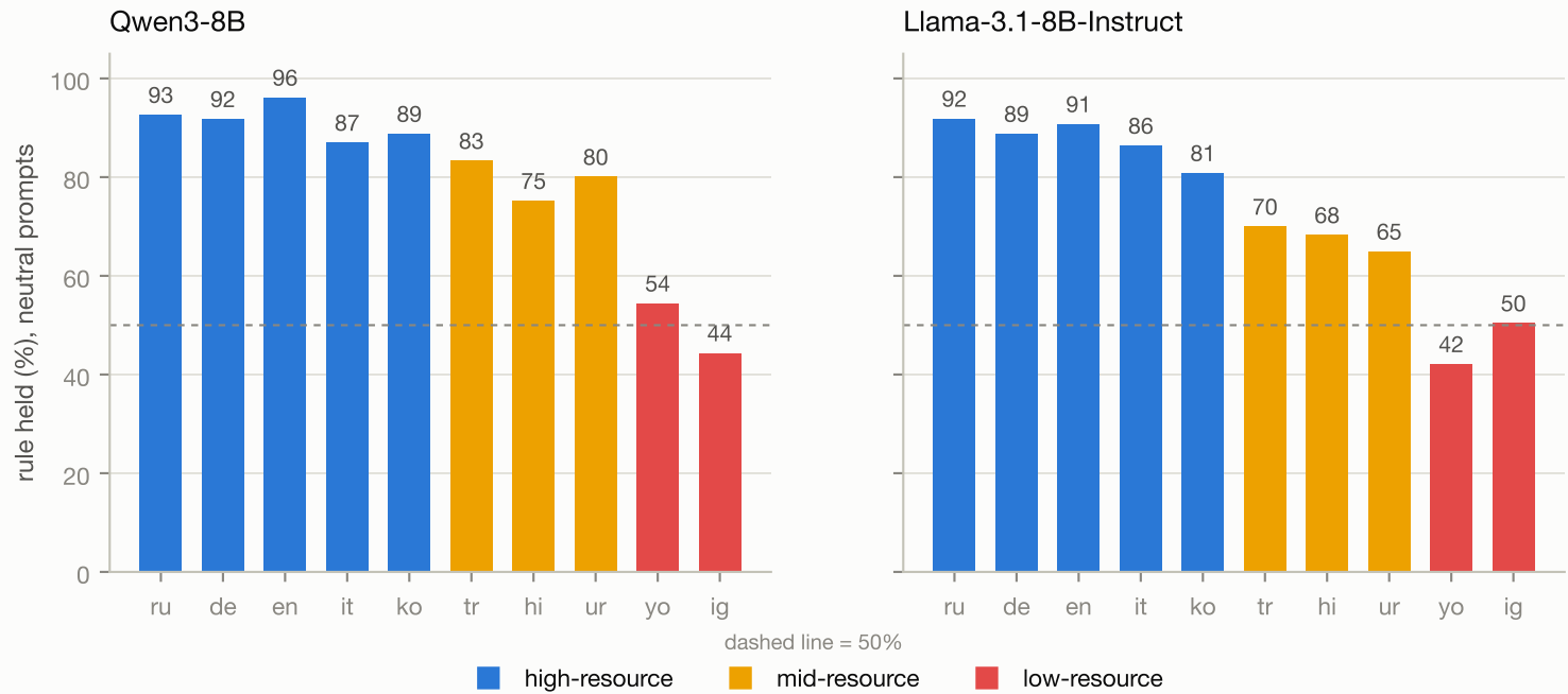
Fig 3 · The same rule, the same task: adherence falls with language resource level
