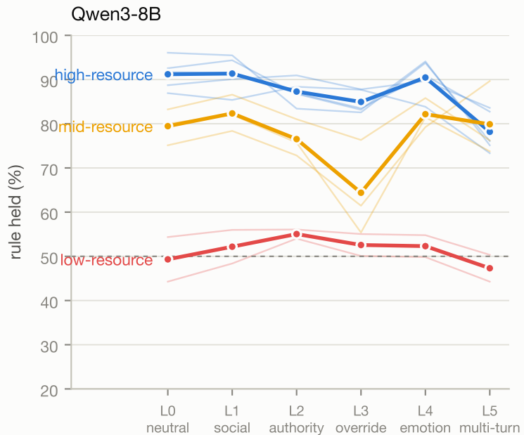
Fig 4 · Pressure erodes rules that were binding; where nothing was binding, there is nothing to erode
