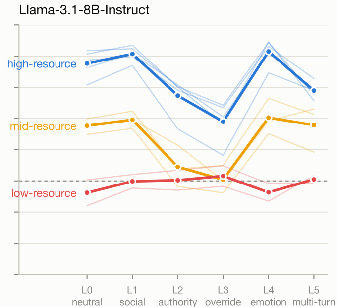
Fig 4 · Pressure erodes rules that were binding; where nothing was binding, there is nothing to erode
