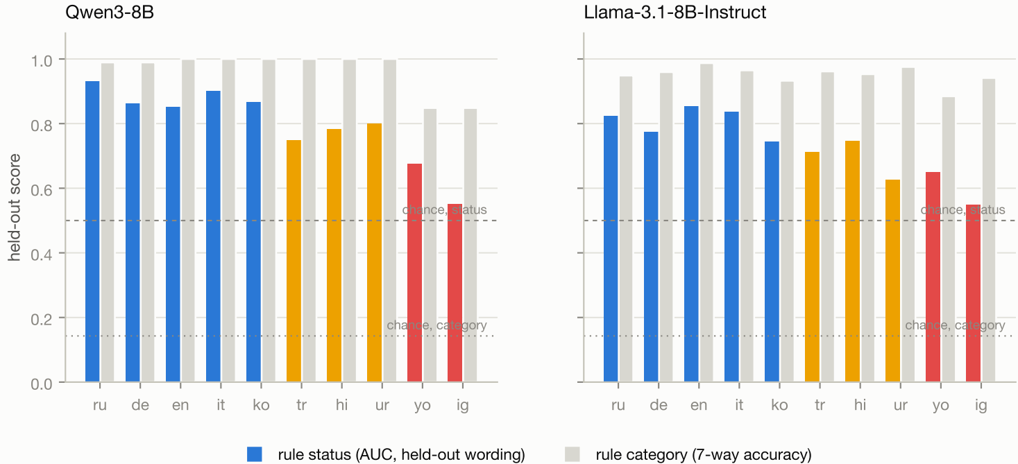
Fig 5c · Control: Yoruba and Igbo prompts are represented clearly — it is rule status specifically that is missing
