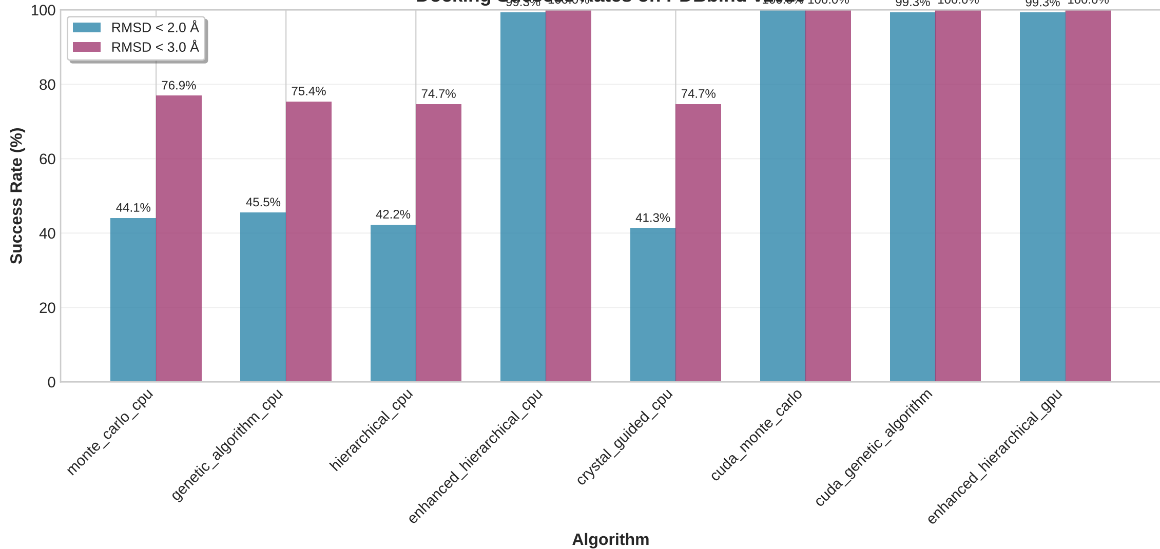
Docking Success Rates on PDBbind v2020
