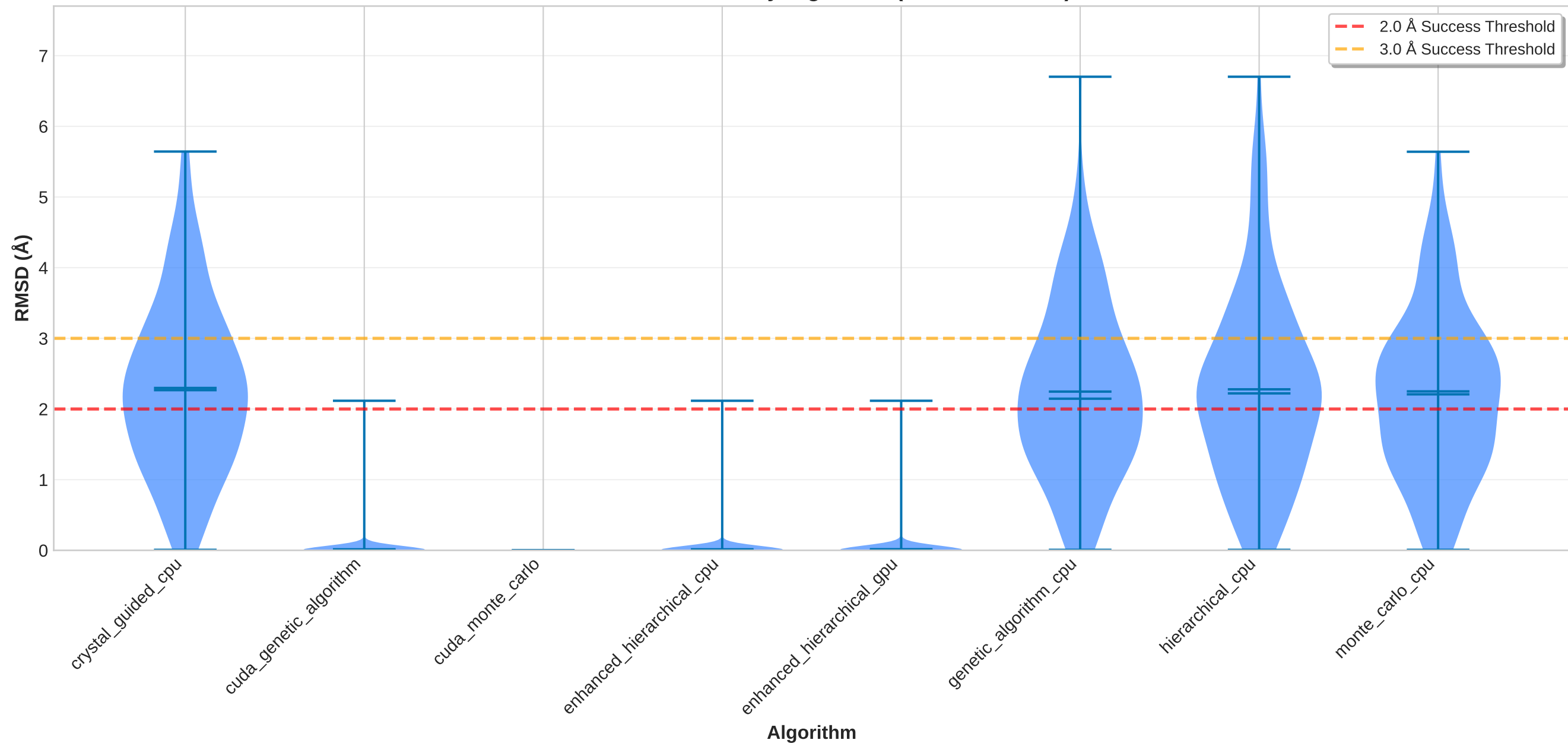
RMSD Distribution by Algorithm (PDBbind v2020)
