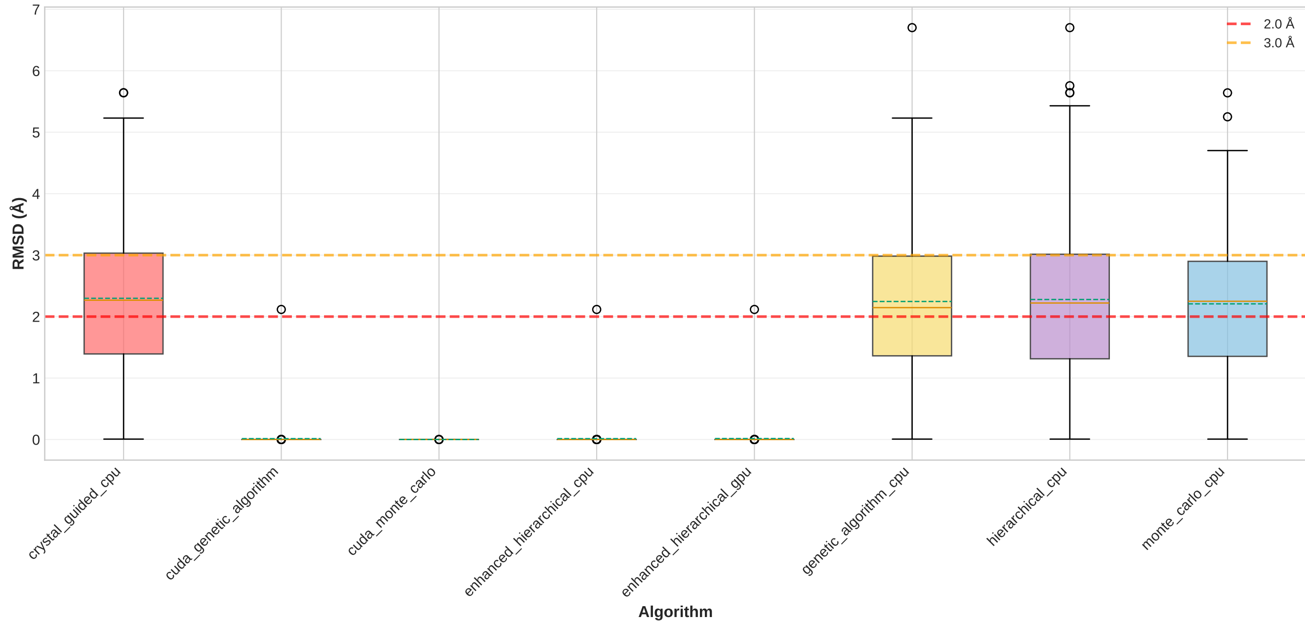
RMSD Box Plot - PDBbind v2020
