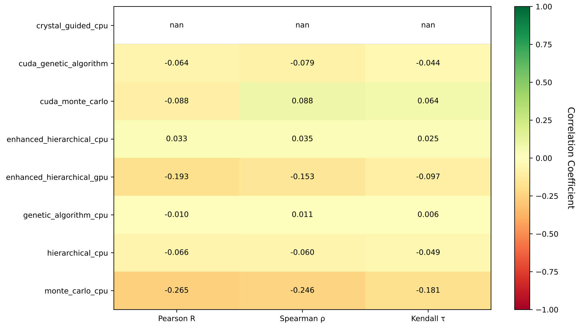
Correlation: Docking Score vs Experimental Binding Affinity
