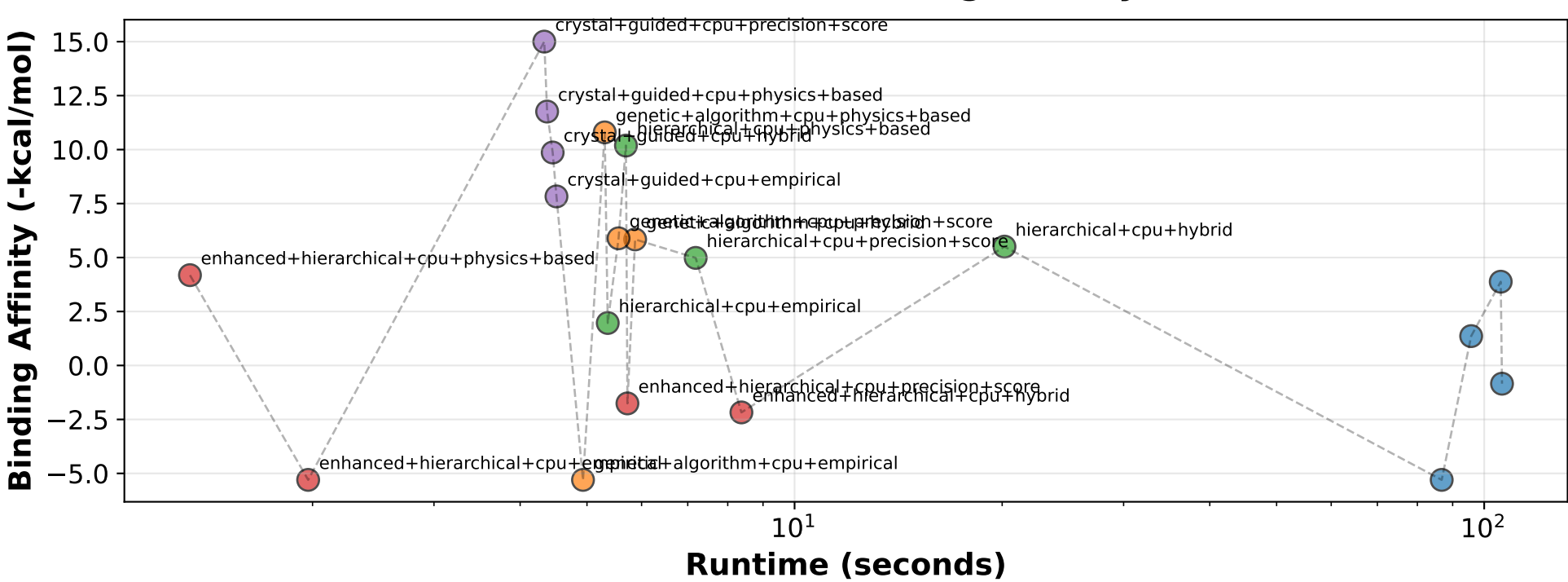
C. Runtime vs Binding Affinity
