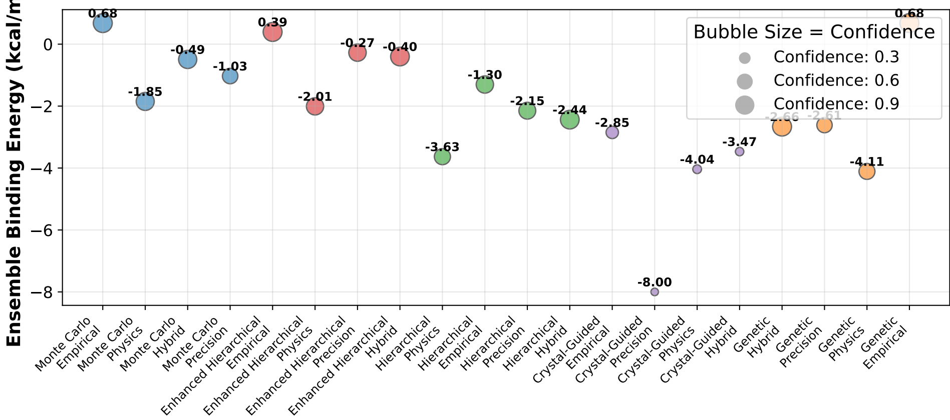
G. Protein-Ligand Interaction Profile
