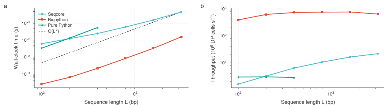
Figure 3: Pairwise global alignment , measured on the AWS g5.2xlarge (AMD EPYC 7R32). a , Wall-clock time against sequence length. Seqcore converges to the O(L^2) reference slope at large L ; at small L it is dominated by fixed per-call NumPy overhead. The scalar Python implementation is omitted above 400 bp, where it becomes impractical. b , The same data as dynamic-programming cell throughput. Seqcore’s throughput rises with L as the fixed cost of each vector operation is amortized over longer anti-diagonals, but plateaus well below Biopython’s compiled aligner.
