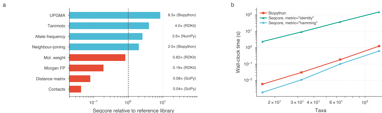
Figure 5: Domain modules against their reference libraries. a , Seqcore relative to the library a user would otherwise use for the same operation, at the largest size measured; the reference is named beside each bar. Bars left of the dashed line are operations where the reference is faster. The molecule functions wrap RDKit and the structural searches wrap a spatial index, so parity rather than advantage is the target there. b , Neighbour-joining against Biopython. The choice of distance metric dominates: identity aligns every pair before building the tree, while hamming compares an already-aligned input column by column. Biopython’s identity calculator does the latter, so only the lower two curves are a like-for-like comparison.
