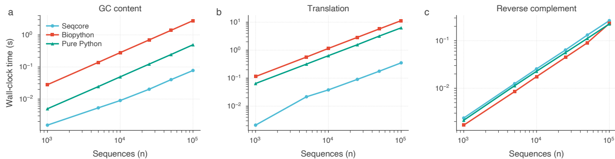
Figure 2: Scaling of batch operations on sequences of 1000 bp, measured on the AWS g5.2xlarge (AMD EPYC 7R32), shown log-log. All implementations are linear in batch size; what differs is the constant factor. a , GC content. b , Translation. c , Reverse complement, where a single compiled pass ( str.translate in Biopython) is already close to the memory-bandwidth limit and Seqcore obtains no advantage.
