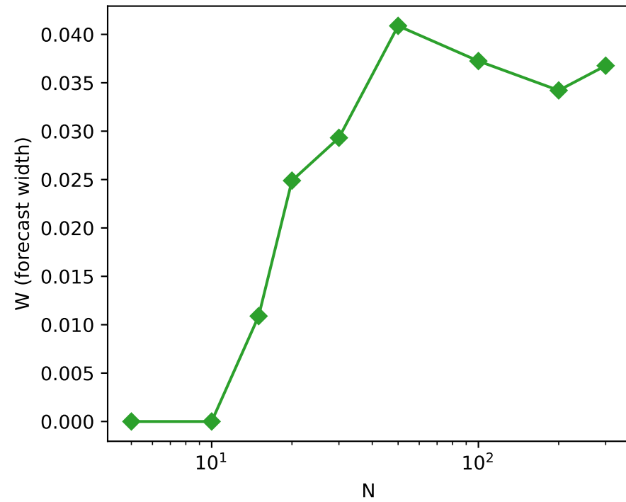
(c) Forecast Width W(N)
