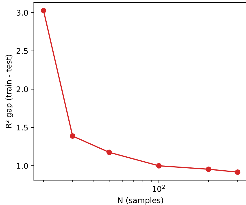
(a) Overfitting Gap vs N
