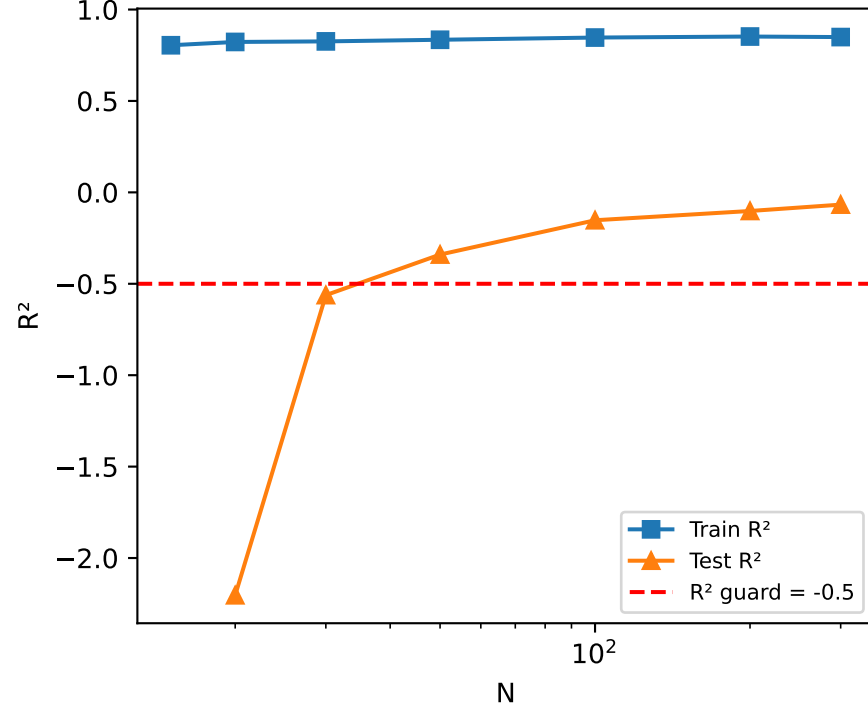
(b) Train vs Test R^2
