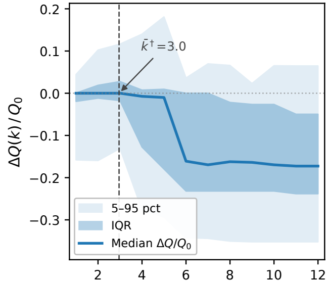
(b) Qwen — 30-session Q envelope
