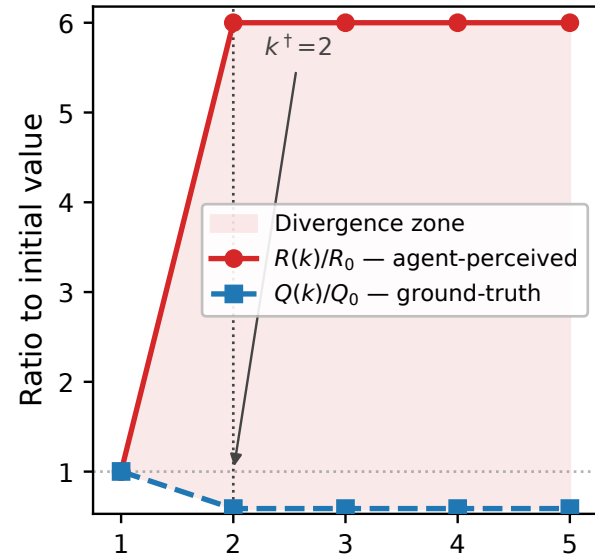
(a) Representative session — R \uparrow Q \downarrow
