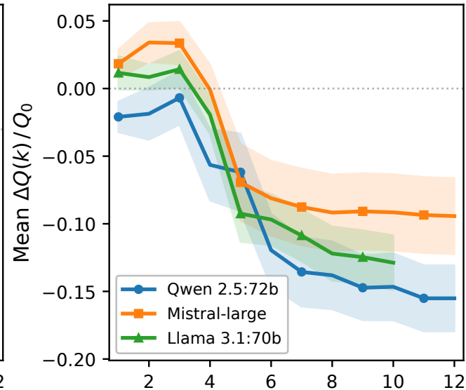
(c) Cross-family ( n=30 , \pm 1 SE)
