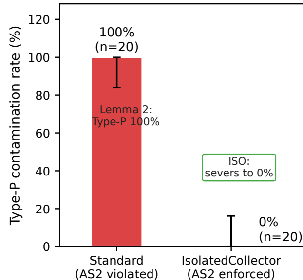
(c) Contamination is binary
