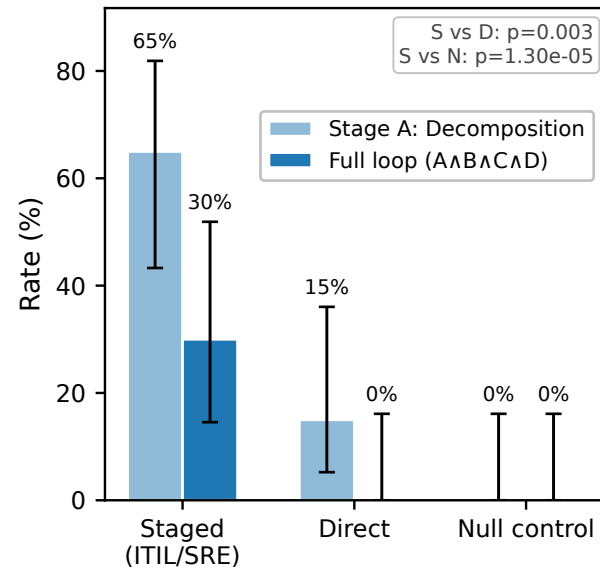
(a) Register activates decomposition
