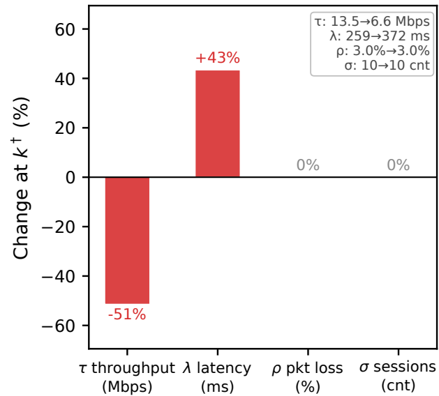
(b) \Phi shifts at k^+ : \tau \downarrow \lambda \uparrow (n=18)
