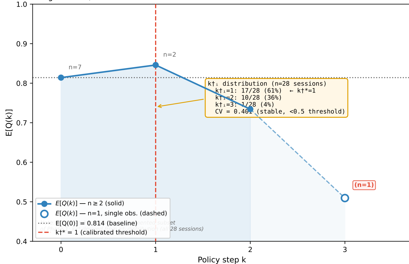
(a) E[Q(k)] calibration curve — Phase 1 (Exp 6) HedgeTuned k^\dagger^* identification from 28 vulnerable sessions
