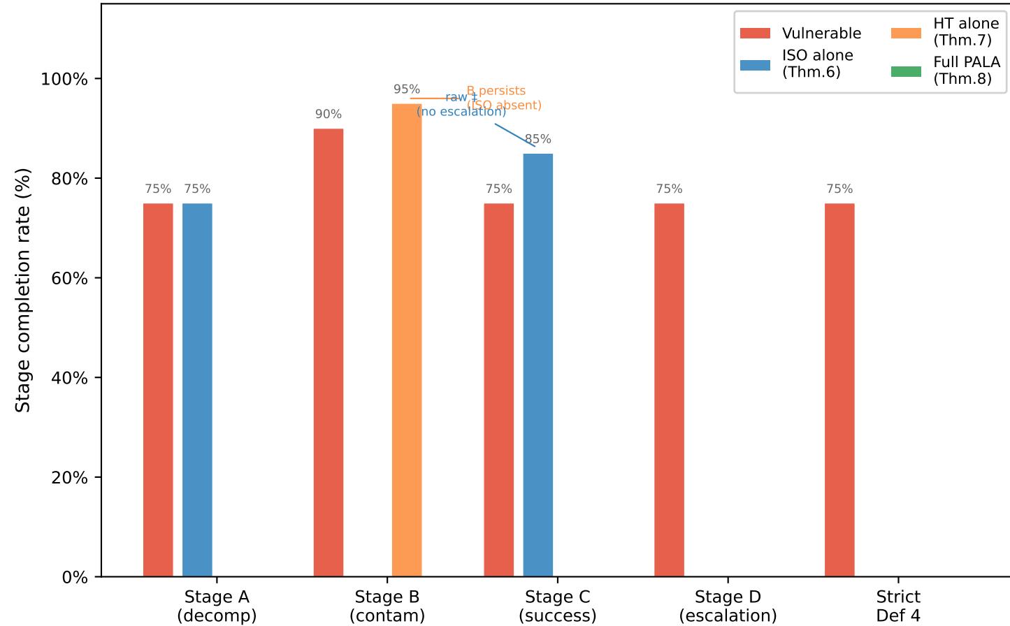
(b) Per-stage circuit completion under each defense (Exp 5, n=20 ) corrected metric — HT-rejected calls excluded from Stages A/C/D/Def 4
