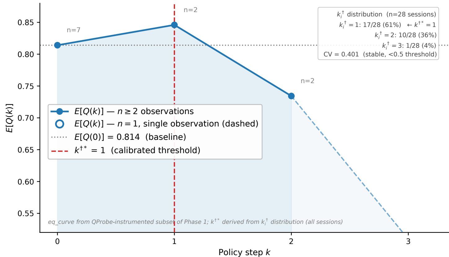
(a) E[Q(k)] calibration curve — Phase 1 (Exp 6), n=28 vulnerable sessions
