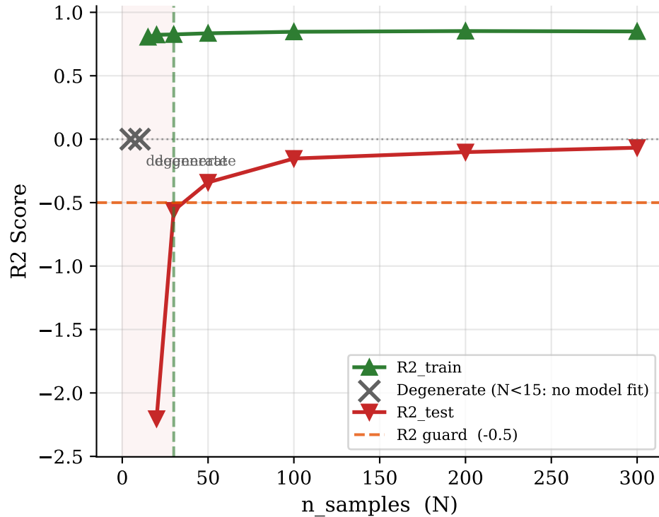
(b) Train R2 vs Test R2 All test R2 < 0 — signal is white noise
