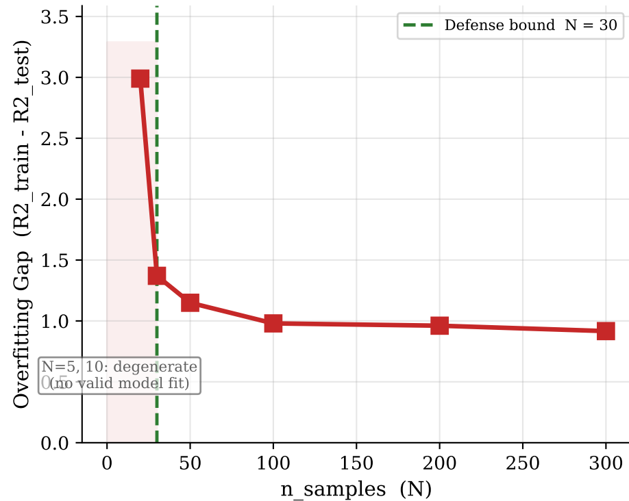
(a) Overfitting Gap vs N Spearman rho = -1.000, p < 0.001
