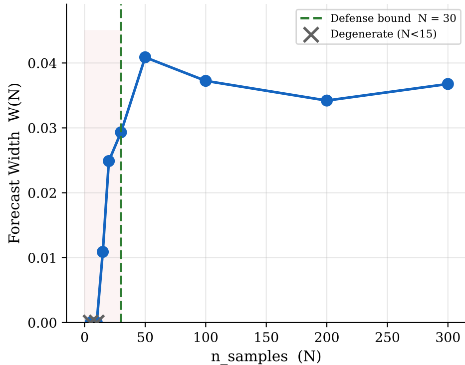
(c) Forecast Width vs N Spearman rho = +0.845, p = 0.004
