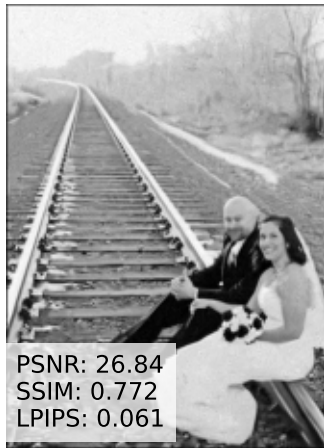
Denoised
