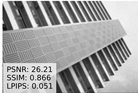
Denoised
