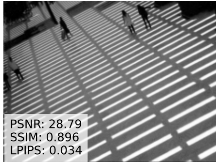
Denoised
