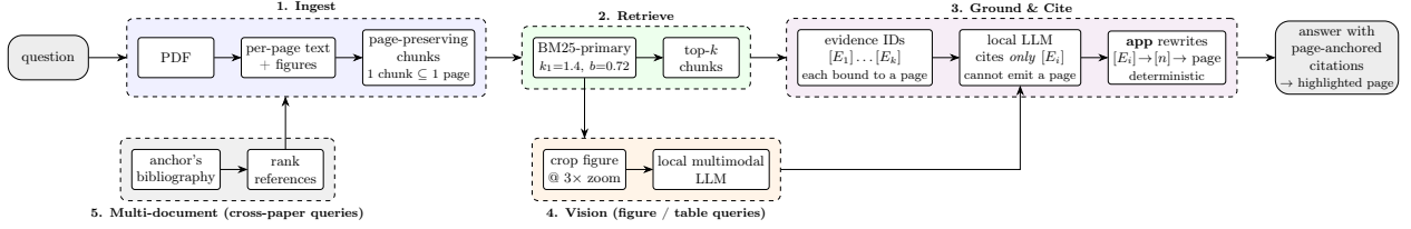
Figure 1: The ScholAR architecture. A question enters at the left and leaves as an answer whose every citation resolves to a highlightable page. (1) Ingest keeps each chunk inside a single PDF page. (2) BM25-primary retrieval returns the top- k chunks. (3) Those chunks are exposed to the model only as evidence identifiers [E_i] , each already bound to the page of the chunk it came from; the model may cite an identifier but can never write a page number, and the application , not the model, rewrites [E_i] into a numbered reference and resolves it to a page. A cited page is therefore correct by construction rather than by the model’s good behavior. (4) Figure and table queries additionally route a cropped, 3 \times -zoomed image to the same local multimodal model. (5) Cross-paper queries first rank the anchor’s bibliography, and the selected reference is then ingested like any other paper. Every component runs on one machine.
