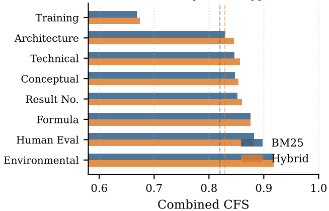
(b) CFS by Claim Type
