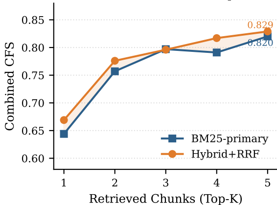
(a) CFS vs. Retrieval Depth
