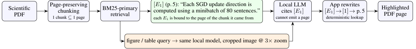
Figure 1: ScholAR’s indirect citation grounding, contrasted with free-form citation. (a) When the model writes the page number itself, the number is generated text: nothing ties it to the passage the model was actually shown. (b) ScholAR keeps every retrieved unit inside one PDF page, exposes the retrieved chunks as evidence identifiers [E_i] that each carry their own page, and permits the model to cite only those identifiers. The application, not the model, rewrites [E_i] into a numbered reference and resolves it to a page, so a cited page is correct by construction. Figure and table queries route to the same local multimodal model with a cropped, 3×-zoomed image. The evidence shown is the real chunk retrieved for this question.
