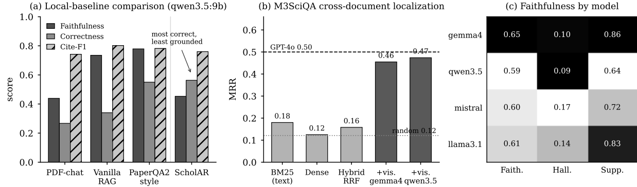
Figure 2: Results at a glance, from the same runs as Tables 7 and 6. (a) On the shared-model local comparison, ScholAR reaches the highest answer correctness (must-include recall) but is among the least faithful under the entailment judge: correctness and grounding come apart. (b) On M3SciQA cross-document localization, resolving the anchor figure with a local multimodal model lifts MRR from the text-only floor (0.18) to near GPT-4o (0.47 vs 0.50), on one laptop. (c) Faithfulness, hallucination, and citation support per generation model (Table 5); shading marks rank within each column (darker is better, with hallucination inverted).
