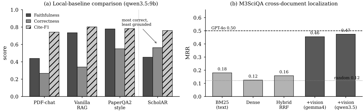
Figure 2: Results at a glance, from the same runs as Tables 7 and 6. (a) On the shared-model local comparison, ScholAR reaches the highest answer correctness but is among the least faithful under the entailment judge: correctness and grounding come apart. (b) On M3SciQA cross-document localization, resolving the anchor figure with a local multimodal model lifts MRR from the text-only floor (0.18) to near GPT-4o (0.47 vs 0.50), on one laptop.
