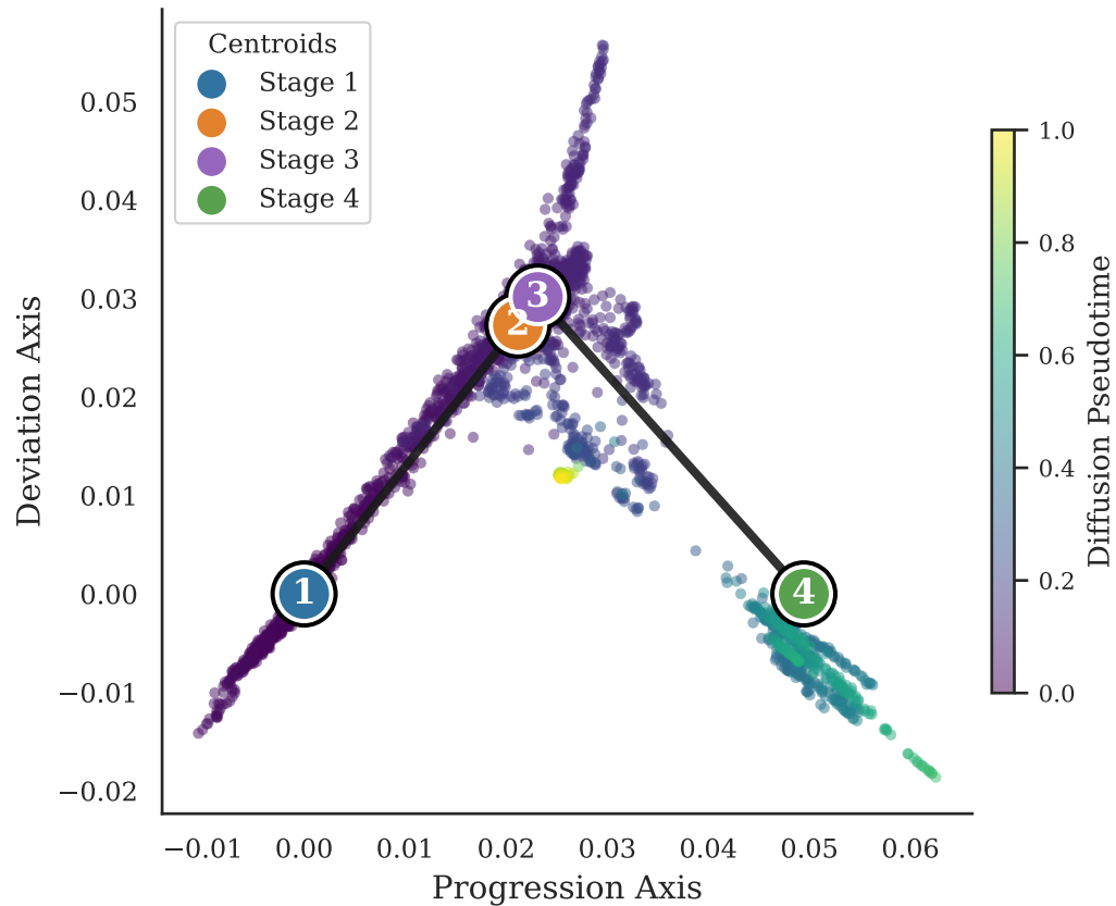
A. Embedding Space: UNI2 on CRC-Conventional
