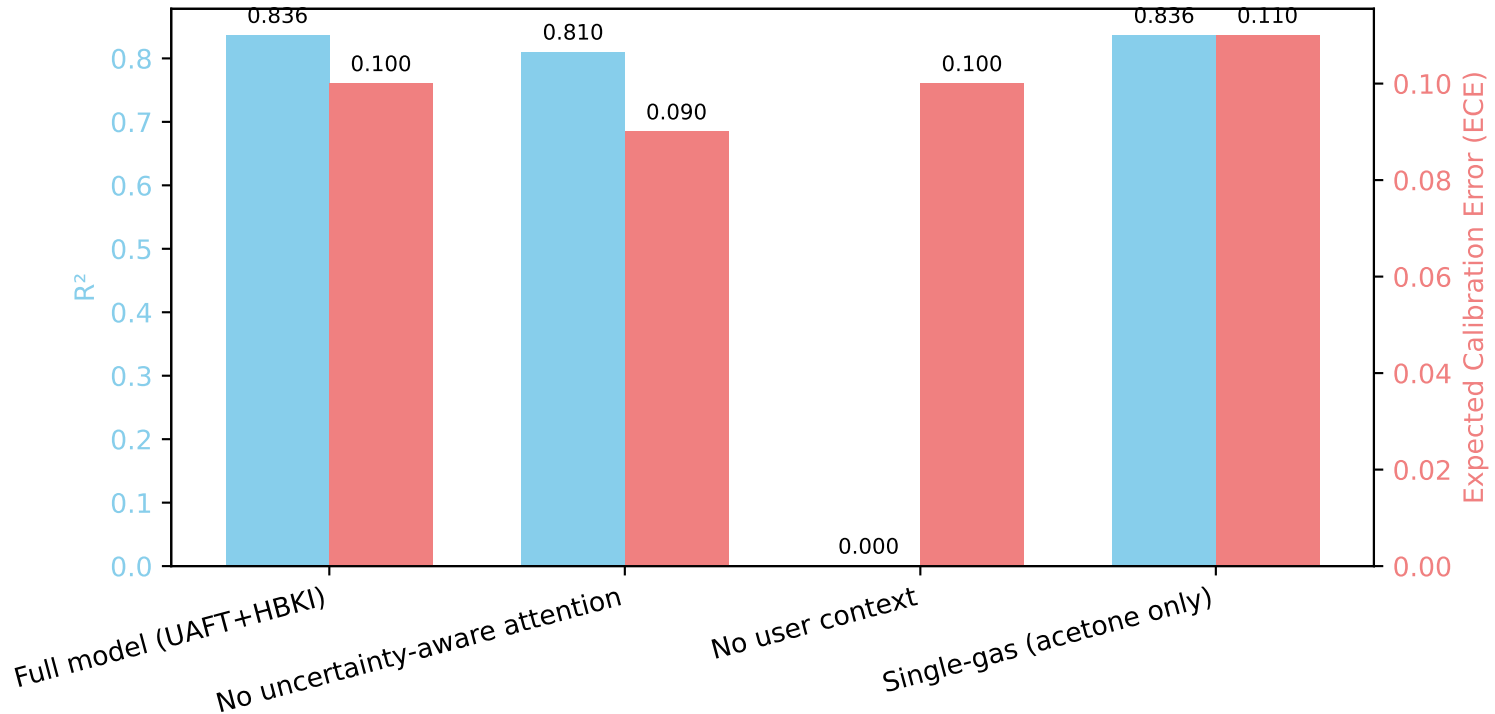
Ablation Study: Impact of Uncertainty-Aware Weighting and User Context
