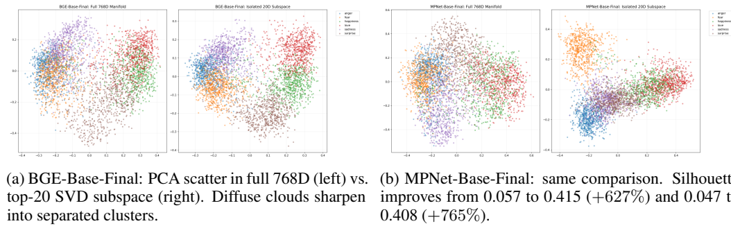
Figure 7: 768D vs. top-20 SVD subspace (Finding 3). Projecting into the 20-dimensional signal subspace reveals the cluster structure hidden by noise dimensions in the full embedding space.
