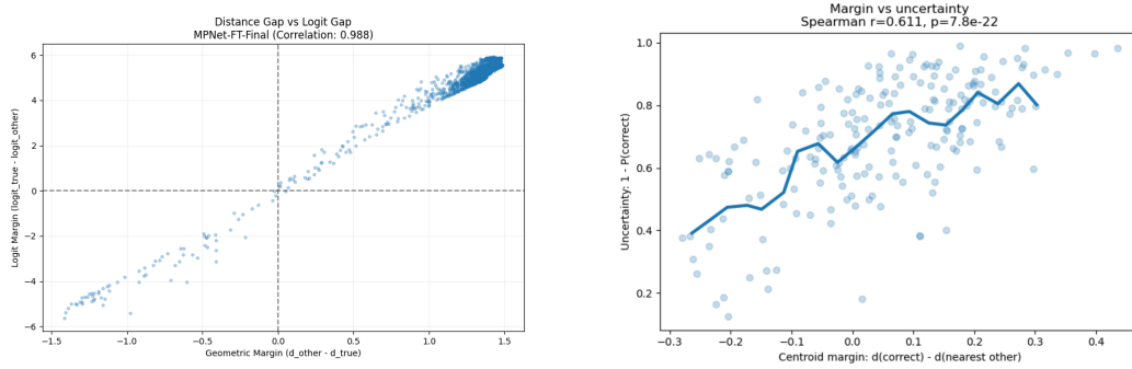
(a) LLM: centroid margin vs. logit margin for MPNet-FT-Final ( r = 0.988 ). Geometric margin almost perfectly determines logit margin.
