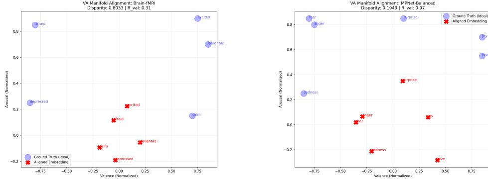
(a) Brain fMRI: poor VA alignment (Disparity=0.80, R_{\text{val}} = 0.31 ). Embeddings (red crosses) deviate markedly from the V-A circumplex (blue circles).
