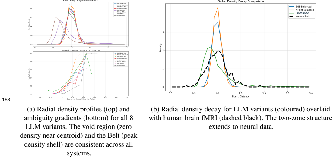
168 (a) Radial density profiles (top) and ambiguity gradients (bottom) for all 8 LLM variants. The void region (zero 169 density near centroid) and the Belt (peak density shell) are consistent across all 170 systems. 171 (b) Radial density decay for LLM variants (coloured) overlaid with human brain fMRI emotion 172 representations, establishing it as a cross-system geometric principle.
