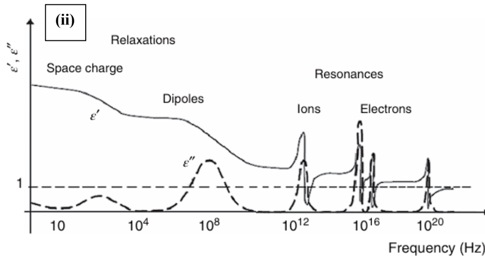
Figure 2.4.2: i) Polarization processes: (a) electronic polarization, (b) ionic polarization, (c) orientational polarization, and (d) space charge polarization. ii) Frequency dependence of polarization dispersion.[25]
