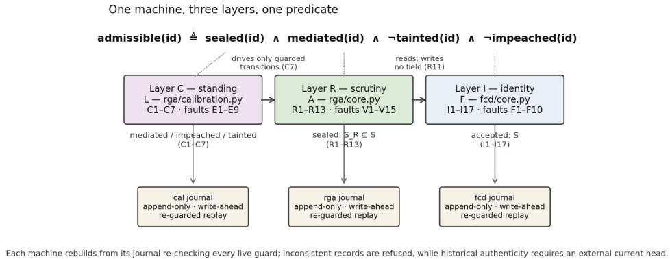
Figure 1: The composed machine. Each conjunct of admissible is the top of one theorem family, and each layer answers exactly one of Section 1’s three questions.
