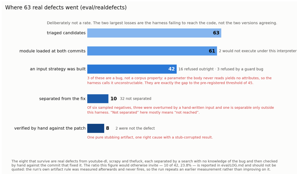
Figure 5: Where the real defects went. The ratio this shape invites — separations over testable — is the one the study’s own log says not to quote, because the run’s artifact rule was measured afterwards and never fires. What the figure reports is the disposition of every candidate and the eight hand-verified separations.
