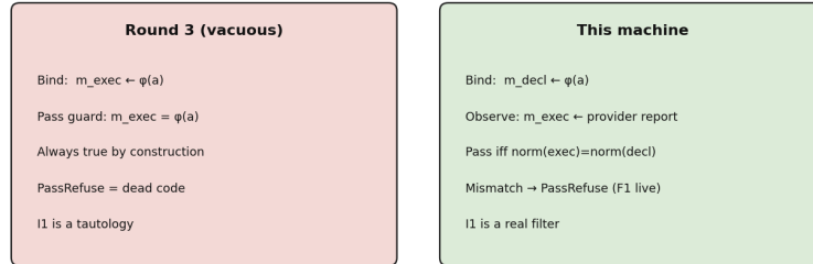
Figure 2: Why I1 is not vacuous. A table in which one transition writes both identities makes the Pass guard a tautology; separating the writers is what gives the guard two independently sourced witnesses to compare, and it is the single most important structural decision in this layer.
