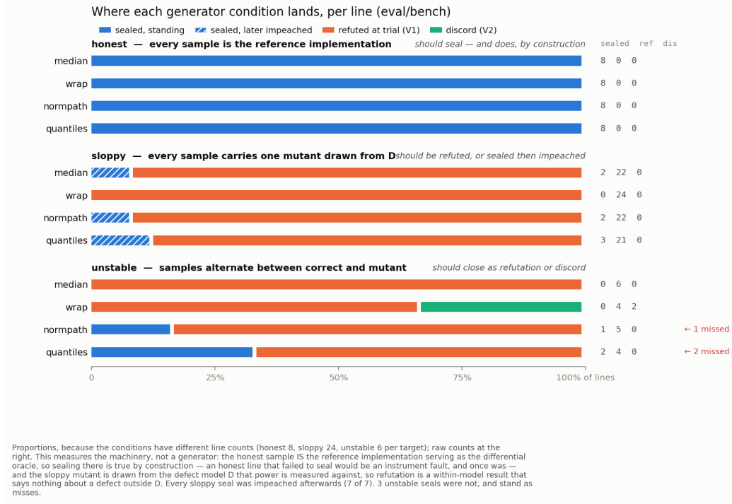
Figure 4: Where each generator condition lands. The figure labels which cells are true by construction rather than leaving the reader to discover it: the honest sample is the differential oracle, and the sloppy mutant is drawn from the very defect model power is measured against. Only the impeachment column is a result.
