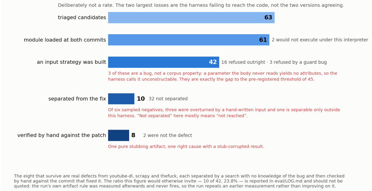
Figure 9. Where 63 real defects went (eval/realdefects)
