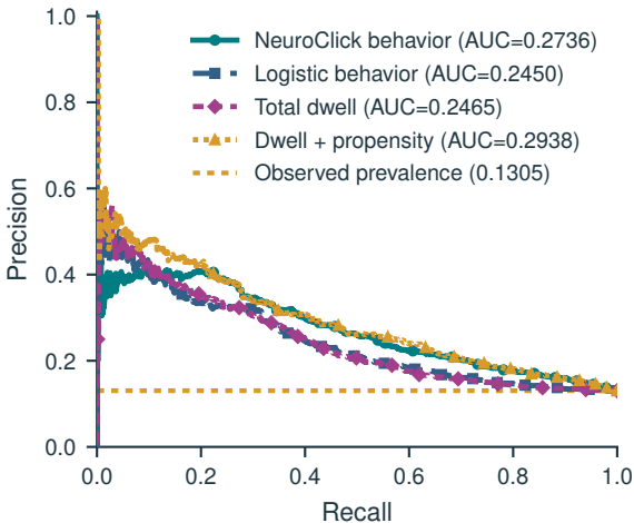
Precision-recall curve
