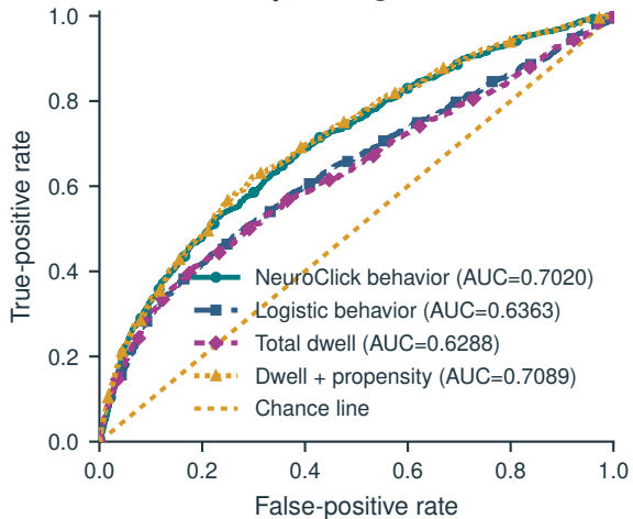
Receiver-operating characteristic
