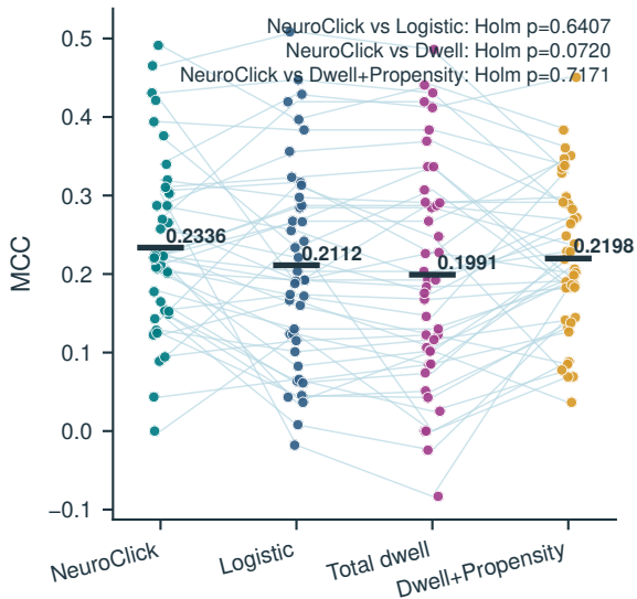
Participant MCC
