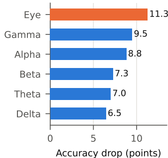
(C) Permutation
