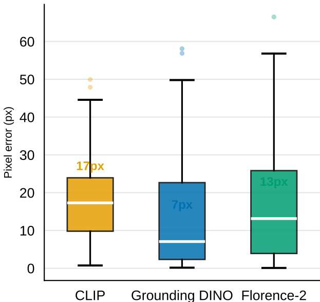
Distribution of localization pixel error — Test Set
