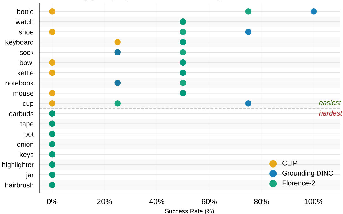
(C) Easy objects favor GDINO, hard objects defeat all models
