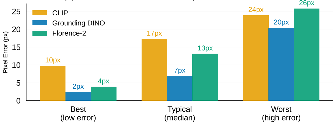
(D) Models show distinct localization precision across all scenarios
