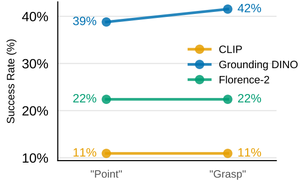
(B) Prompt phrasing effect on model accuracy
