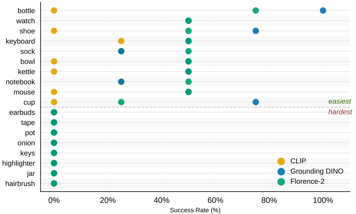
(C) Easy objects favor GDINO, hard objects defeat all models
