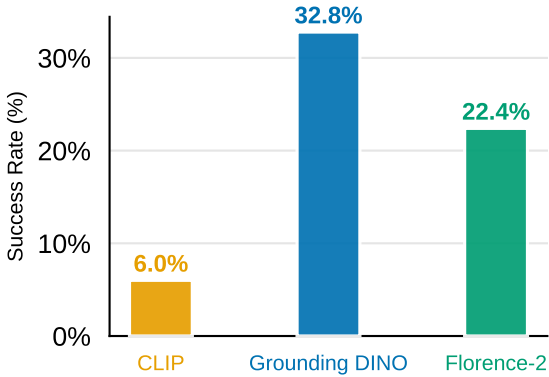
(A) Detection-based models dominate grasp localization
