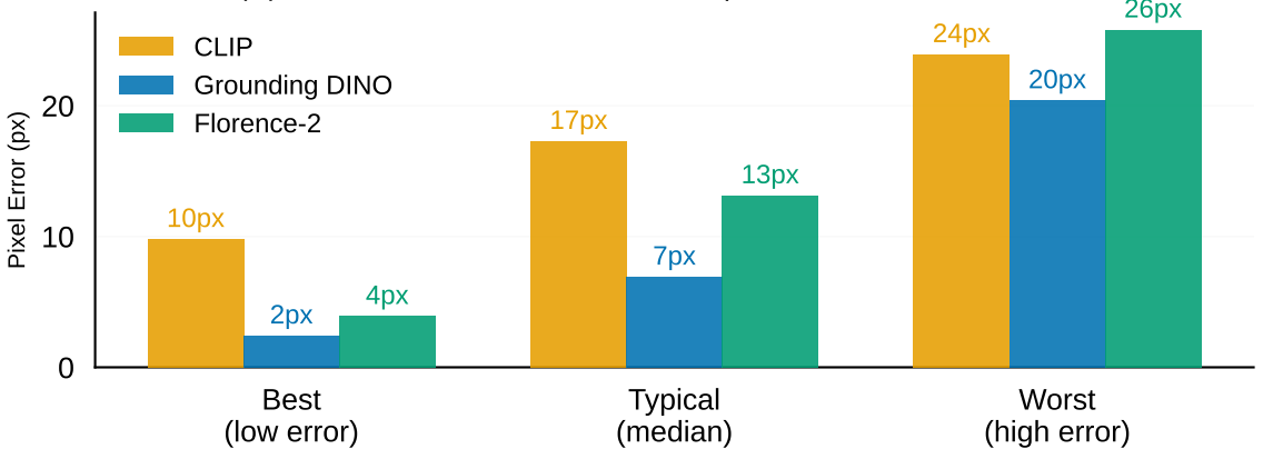
(D) Models show distinct localization precision across all scenarios
