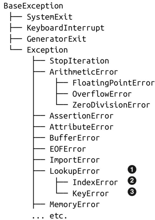
Figure 13-6. Part of the Exception class hierarchy. 11
