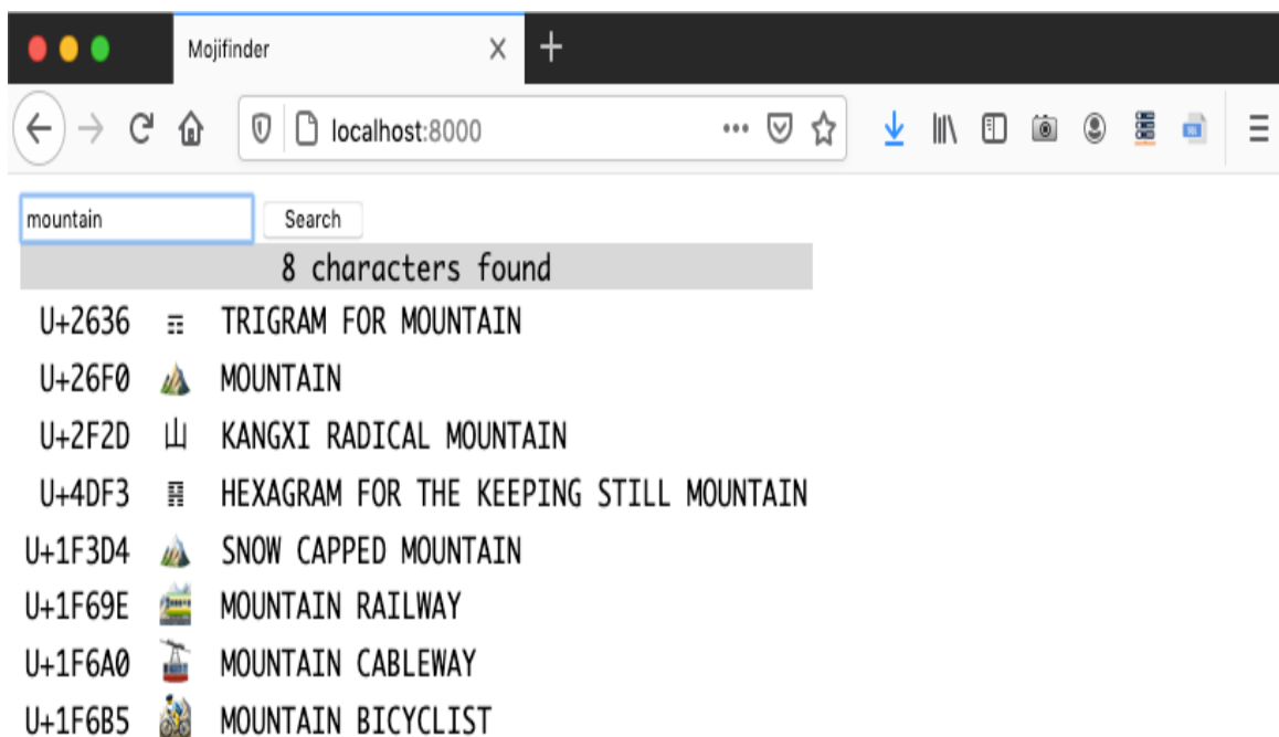
Figure 21-2. Browser window displaying search results for “mountain” from the web_mojifinder.py service.
