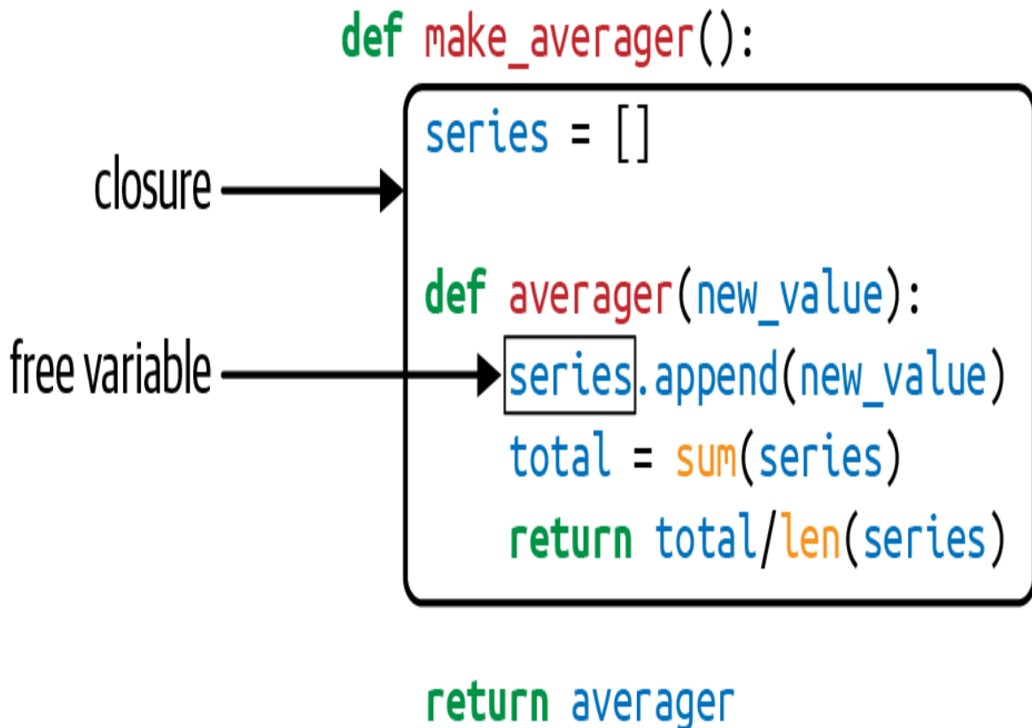
Figure 9-1. The closure for averager extends the scope of that function to include the binding for the free variable series .
