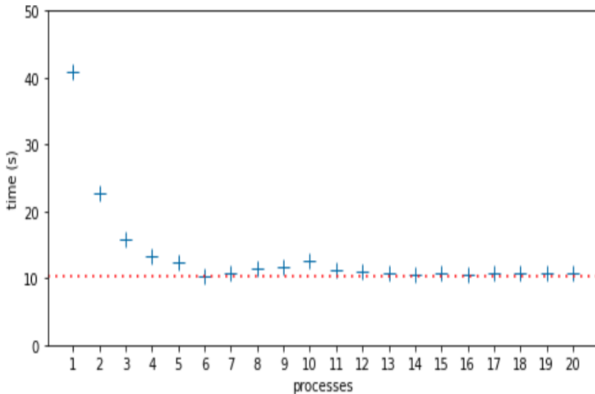
Figure 19-2. Median run times for each number of processes from 1 to 20. Highest median time was 40.81s, with 1 process. Lowest median time was 10.39s, with 6 processes, indicated by the dotted line.
