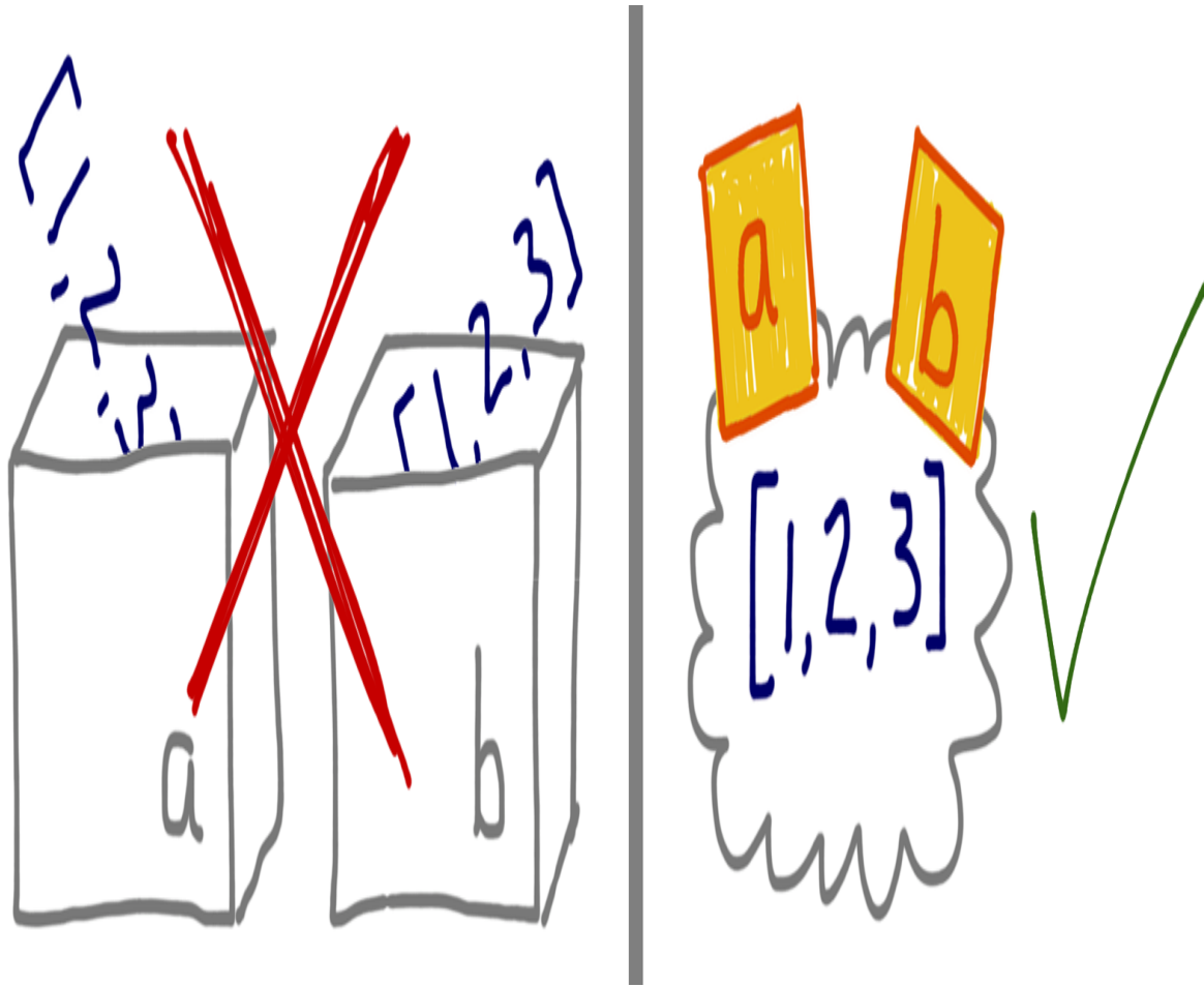
Figure 6-1. If you imagine variables are like boxes, you can't make sense of assignment in Python; instead, think of variables as sticky notes, and Example 6-1 becomes easy to explain.
