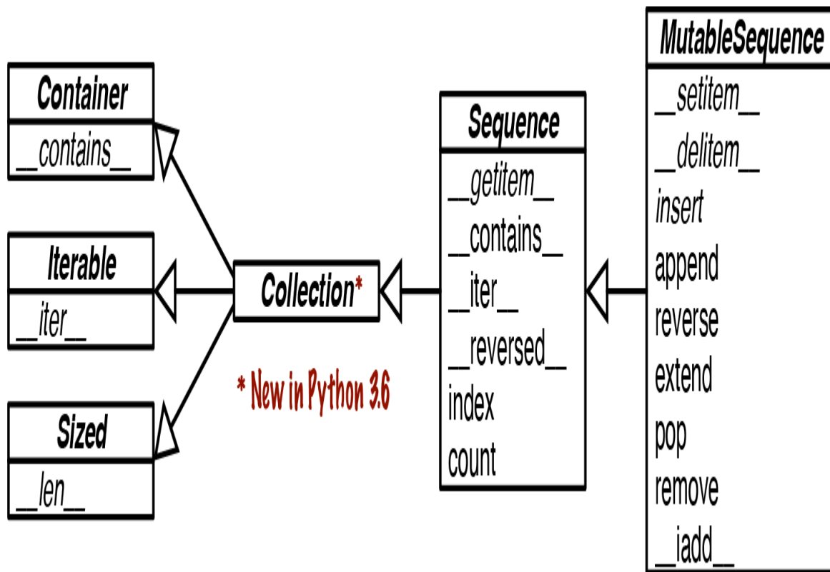
Figure 13-3. UML class diagram for the MutableSequence ABC and its superclasses from collections.abc (inheritance arrows point from subclasses to ancestors; names in italic are abstract classes and abstract methods).
