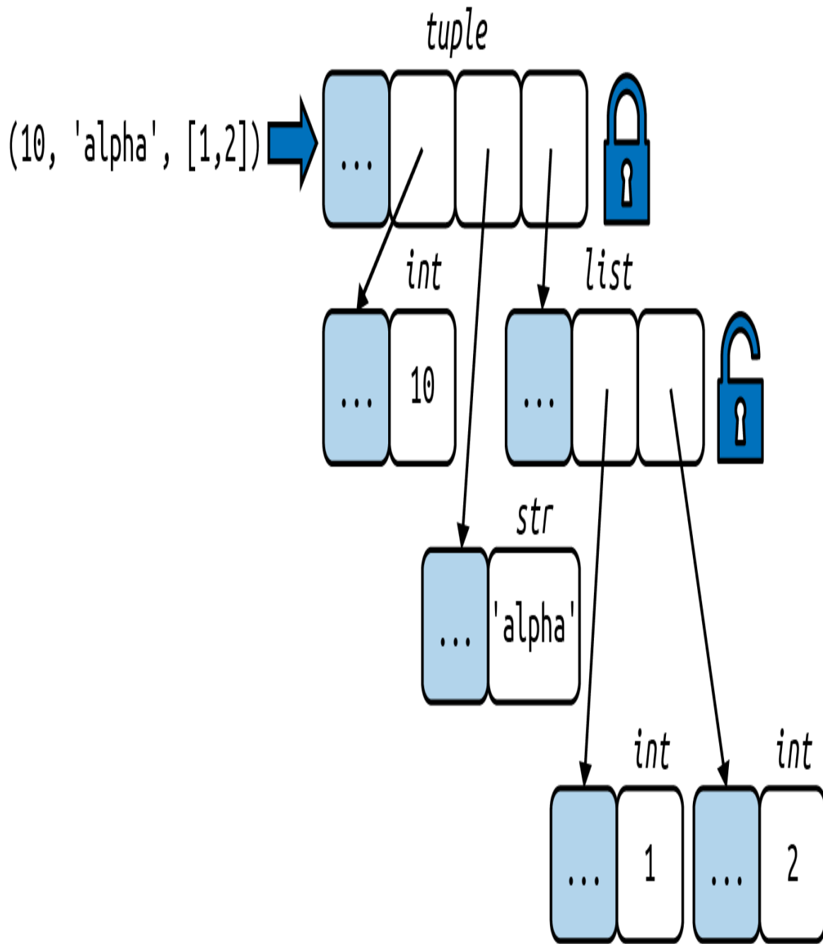
Figure 2-4. The content of the tuple itself is immutable, but that only means the references held by the tuple will always point to the same objects. However, if one of the referenced objects is mutable—like a list—its content may change.
