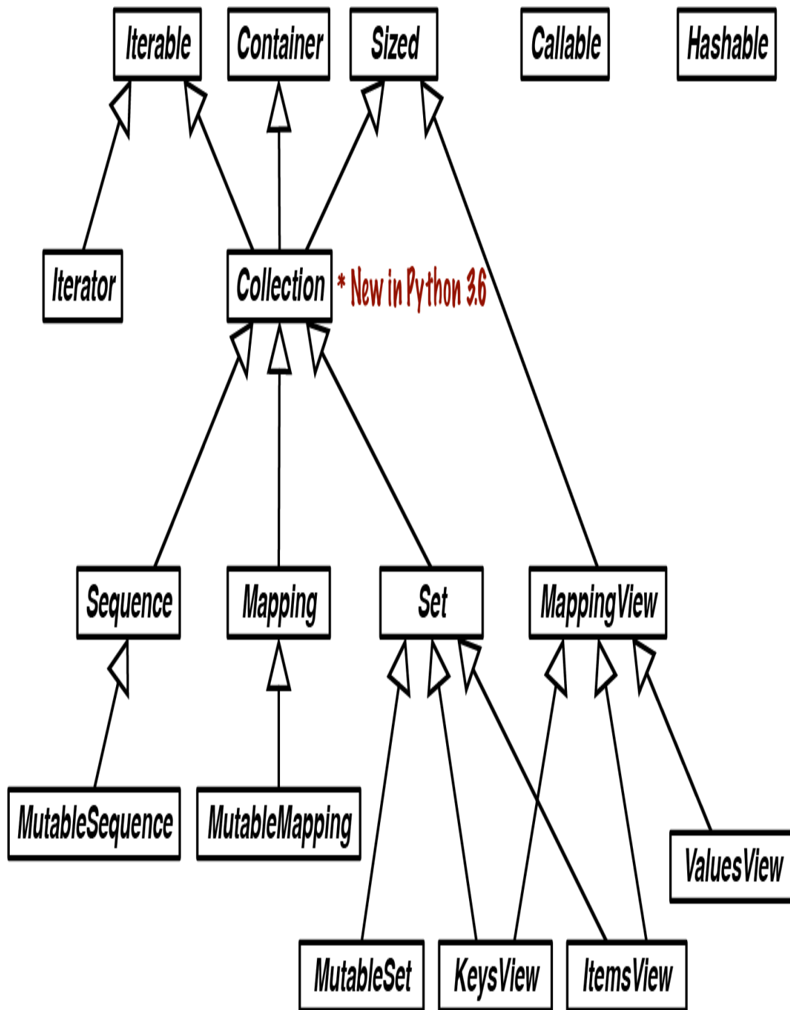
Figure 13-4. UML class diagram for ABCs in collections.abc .
