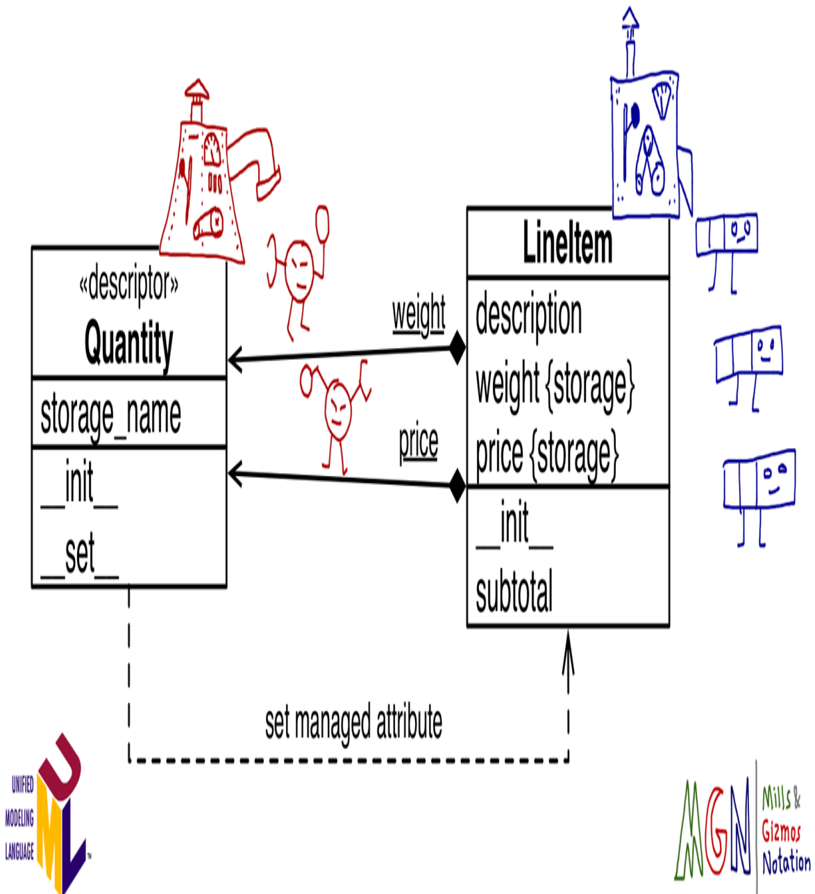
Figure 23-2. UML class diagram annotated with MGN (Mills & Gizmos Notation): classes are mills that produce gizmos—the instances. The Quantity mill produces two gizmos with round heads, which are attached to the LineItem mill: weight and price . The LineItem mill produces rectangular gizmos that have their own weight and price attributes where those values are stored.
