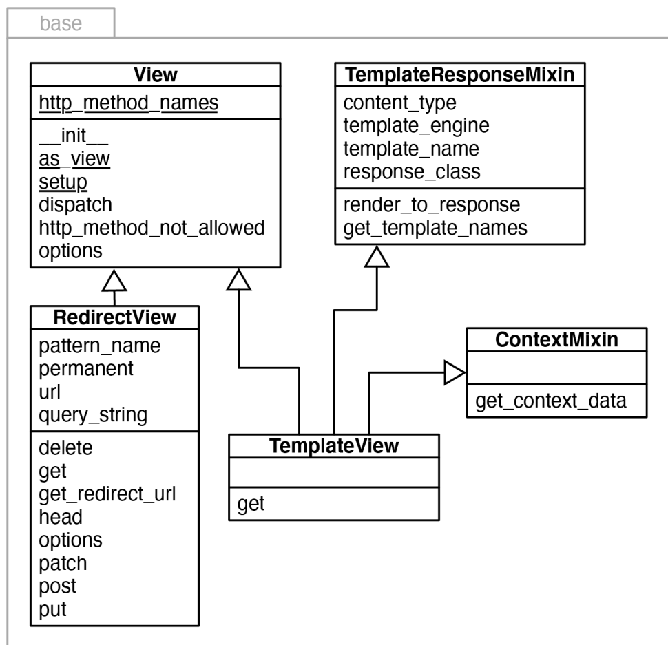
Figure 14-3. UML class diagram for the django.views.generic.base module.
