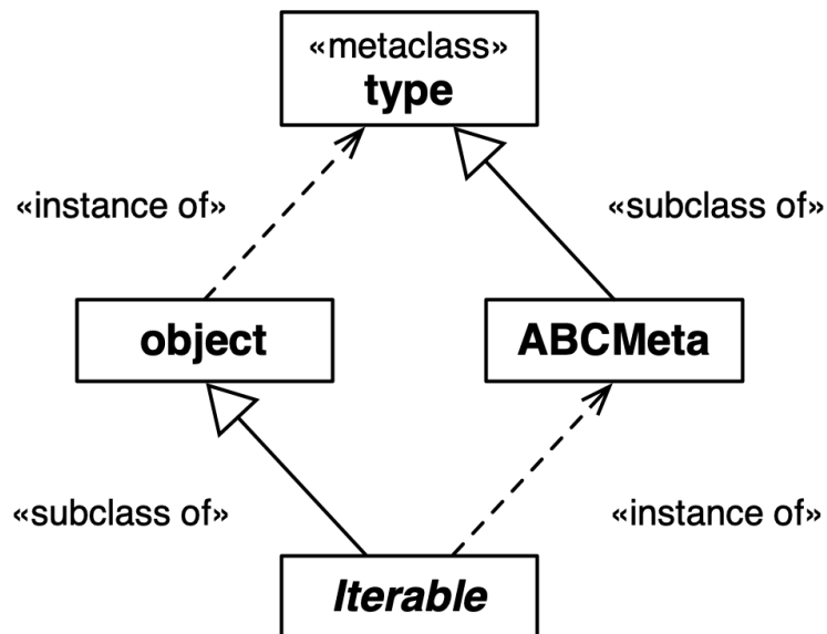
Figure 24-3. Iterable is a subclass of object and an instance of ABCMeta . Both object and ABCMeta are instances of type , but the key relationship here is that ABCMeta is also a subclass of type , because ABCMeta is a metaclass. In this diagram, Iterable is the only abstract class.
