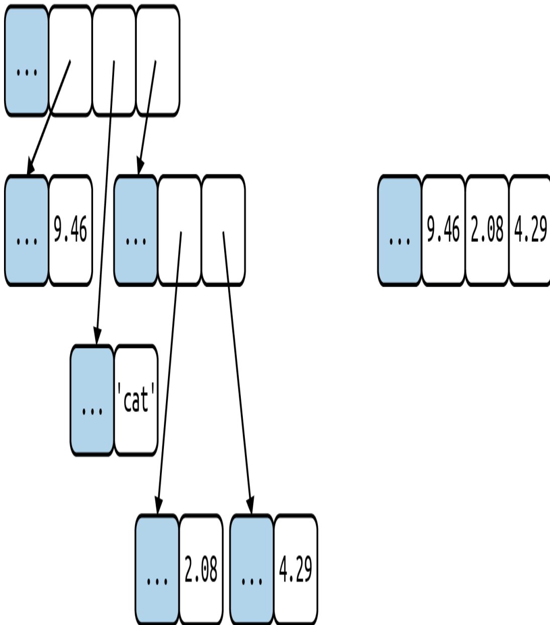
Figure 2-1. Simplified memory diagrams for a tuple and an array , each with three items. Gray cells represent the in-memory header of each Python object—not drawn to proportion. The tuple has an array of references to its items. Each item is a separate Python object, possibly holding references to other Python objects, like that two-item list. In contrast, the Python array is a single object, holding a C language array of three doubles.
