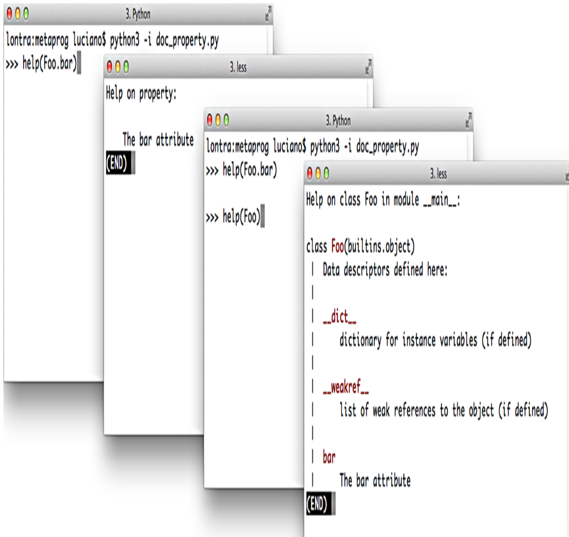
Figure 22-1. Screenshots of the Python console when issuing the commands help(Foo.bar) and help(Foo) . Source code is in Example 22-26 .
