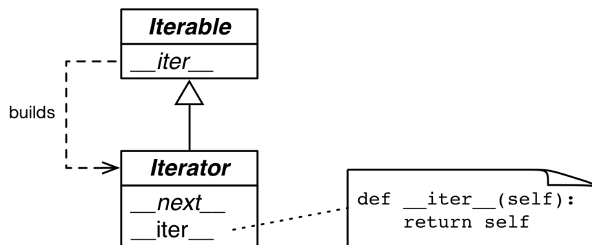
Figure 17-1. The Iterable and Iterator ABCs. Methods in italic are abstract. A concrete Iterable.__iter__ should return a new Iterator instance. A concrete Iterator must implement __next__ . The Iterator.__iter__ method just returns the instance itself.
