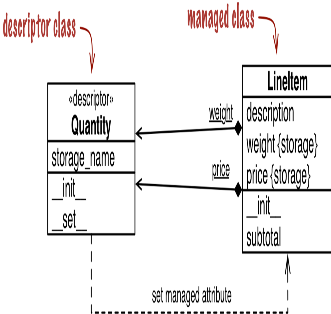
Figure 23-1. UML class diagram for LineItem using a descriptor class named Quantity . Underlined attributes in UML are class attributes. Note that weight and price are instances of Quantity attached to the LineItem class, but LineItem instances also have their own weight and price attributes where those values are stored.
