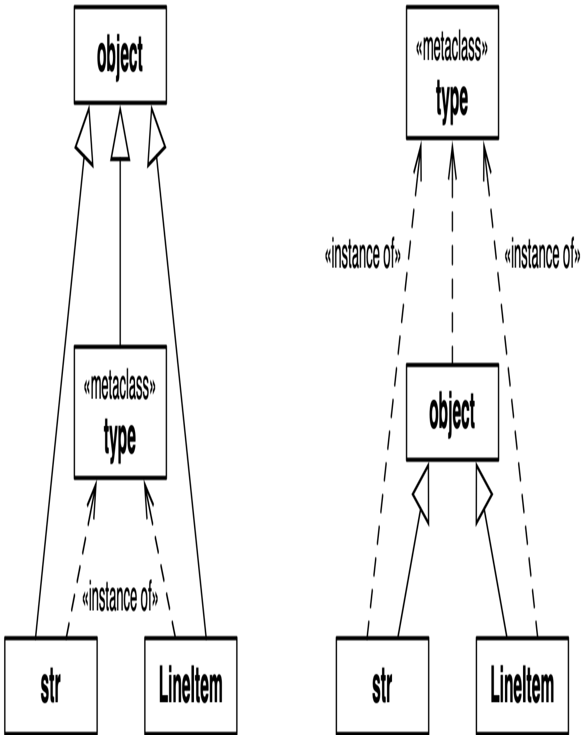
Figure 24-2. Both diagrams are true. The left one emphasizes that str , type , and LineItem are subclasses of object . The right one makes it clear that str , object , and LineItem are instances of type , because they are all classes.
