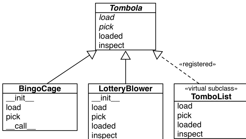
Figure 13-5. UML diagram for an ABC and three subclasses. The name of the Tombola ABC and its abstract methods are written in italics, per UML conventions. The dashed arrow is used for interface implementation—here I am using it to show that TomboList not only implements the Tombola interface, but is also registered as virtual subclass of Tombola —as we will see later in this chapter. 9
