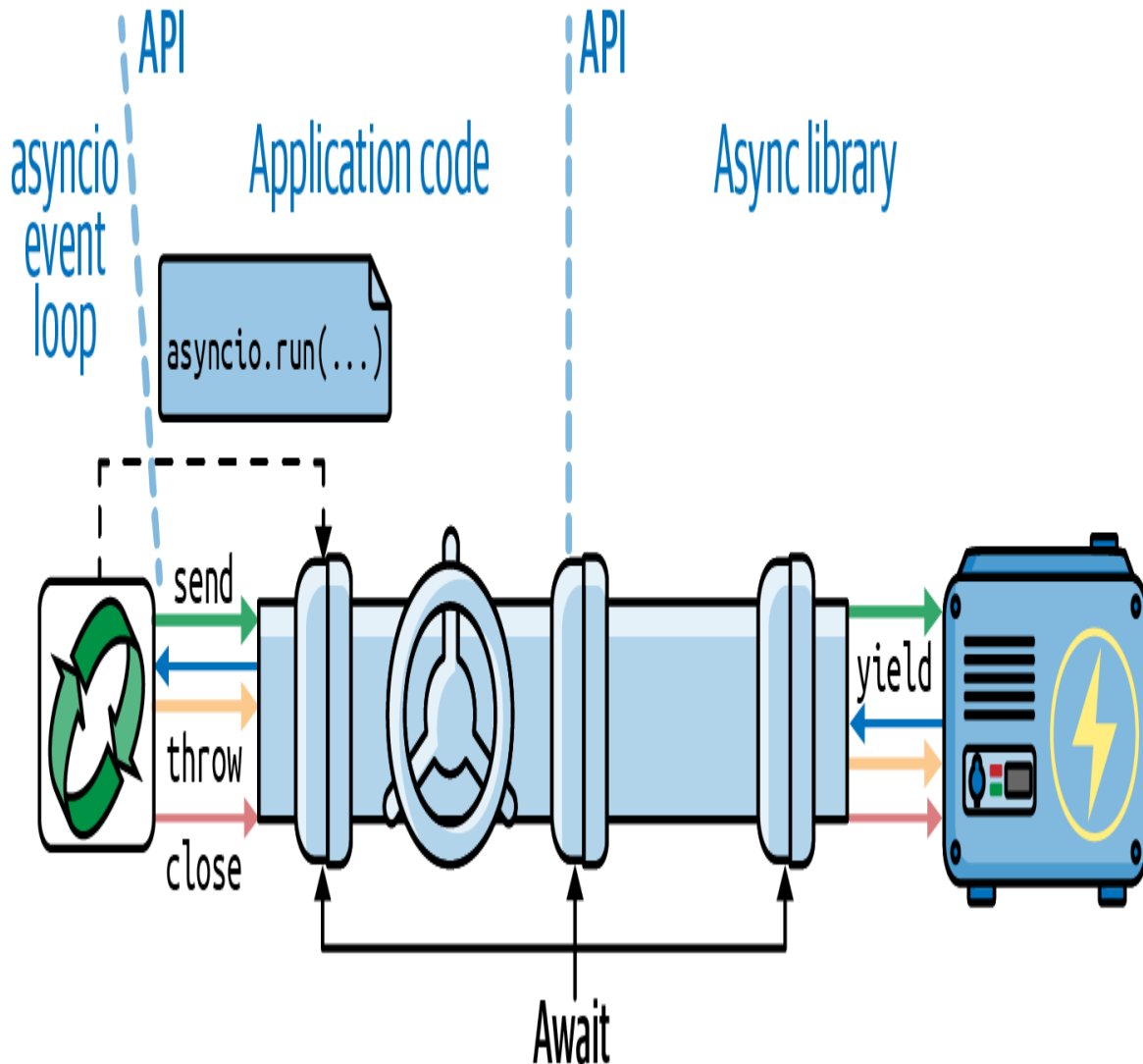
Figure 21-1. In an asynchronous program, a user's function starts the event loop, scheduling an initial coroutine with asyncio.run(...) . Each user's coroutine drives the next with an await expression, forming a channel that enables communication between a library like HTTPX and the event loop.
