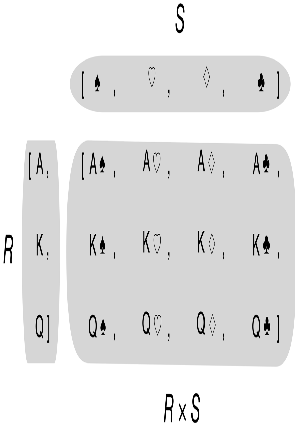
Figure 2-3. The Cartesian product of 3 card ranks and 4 suits is a sequence of 12 pairings.
