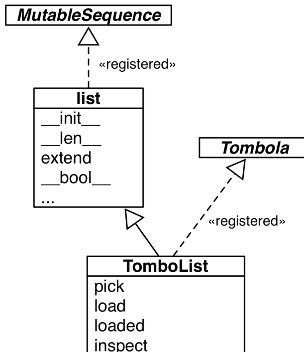
Figure 13-7. UML class diagram for the TomboList , a real subclass of list and a virtual subclass of Tombola .
