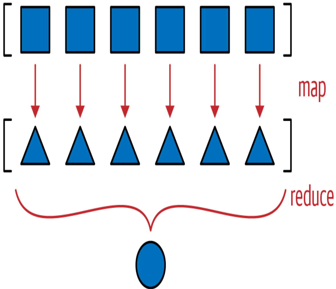
Figure 12-2. Map-reduce: apply function to each item to generate a new series (map), then compute the aggregate (reduce).
