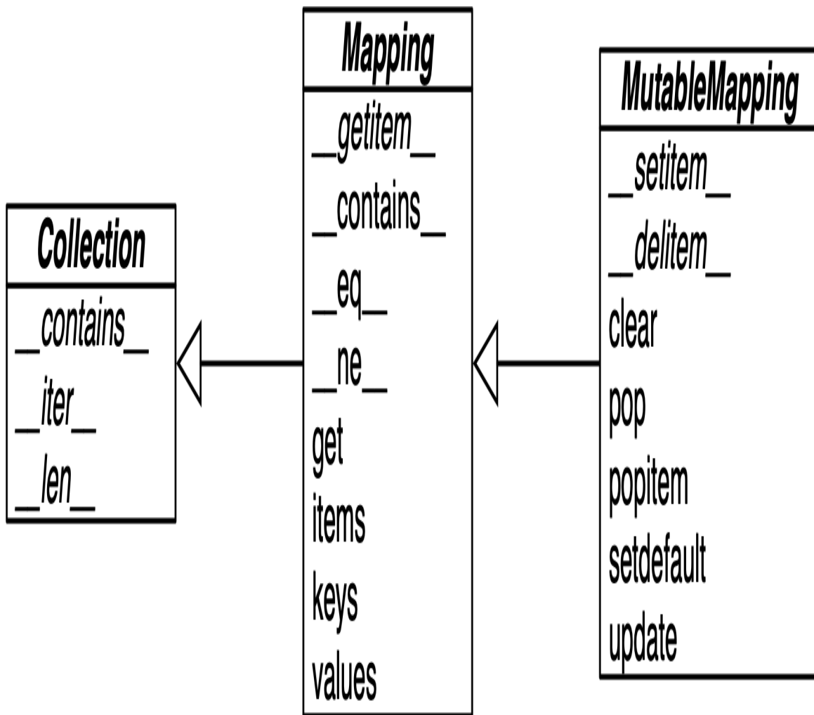
Figure 3-1. Simplified UML class diagram for the MutableMapping and its superclasses from collections.abc (inheritance arrows point from subclasses to superclasses; names in italics are abstract classes and abstract methods).
