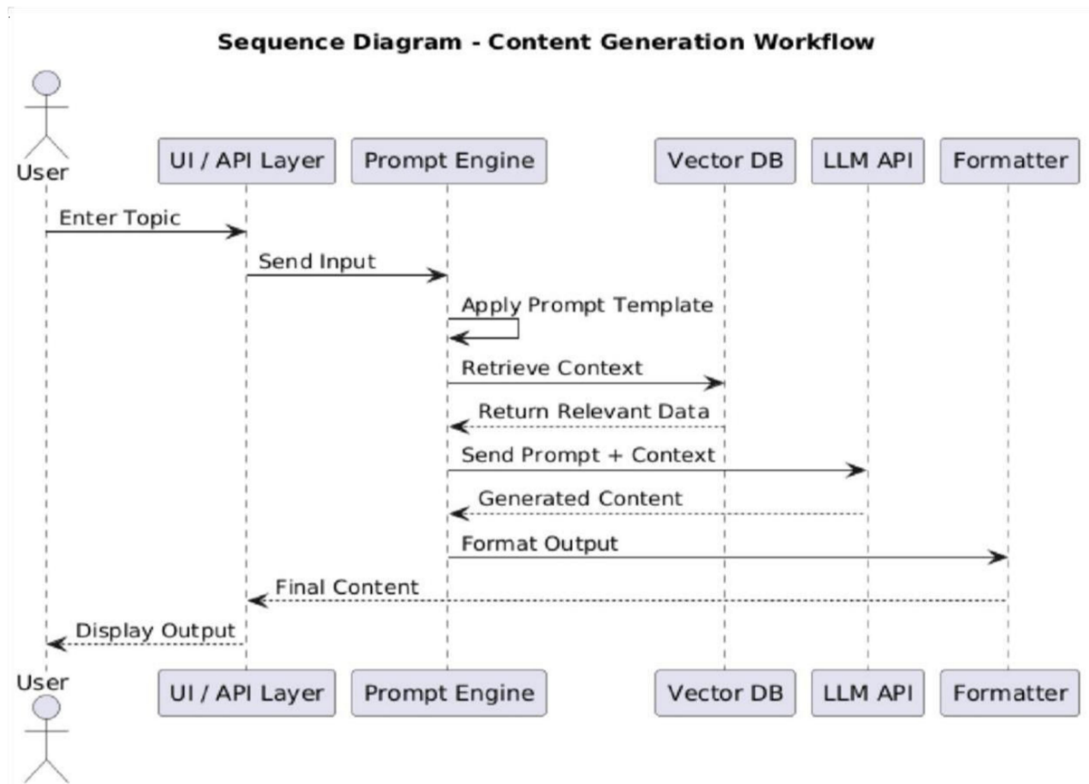
Figure 3: Sequence Diagram
