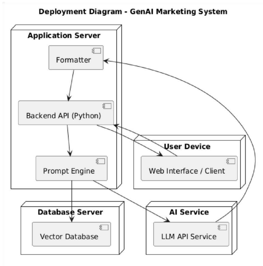
Figure 5: Deployment Diagram
