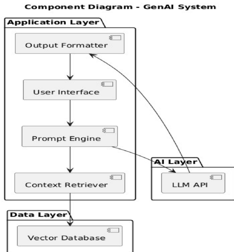
Figure 2: Component Diagram
