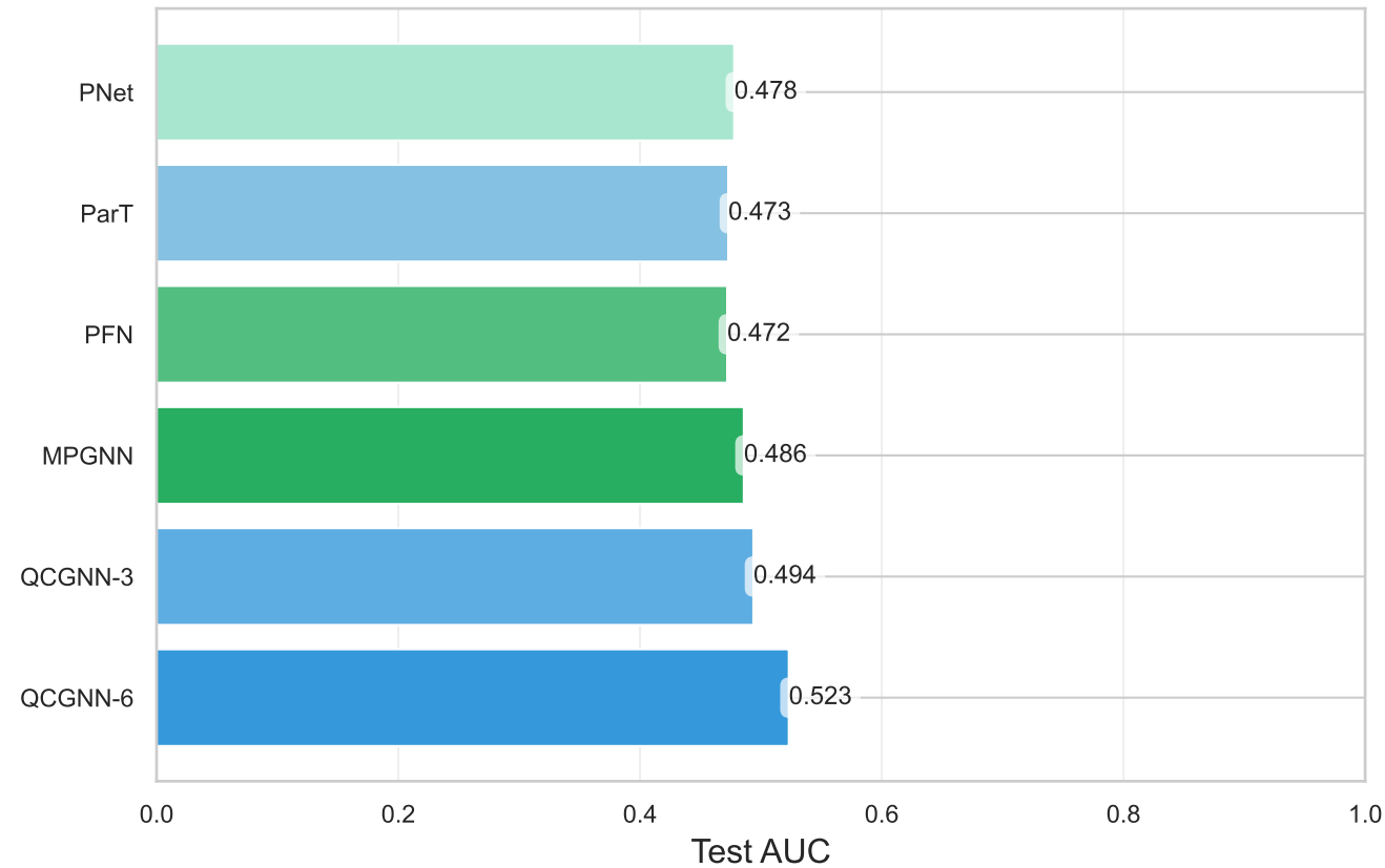
Model Comparison - AUC (Quick Train: 250 samples/class, 1 epoch)
