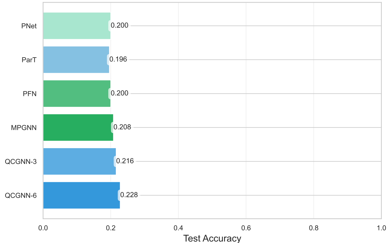
Model Comparison - Accuracy (Quick Train: 250 samples/class, 1 epoch)
