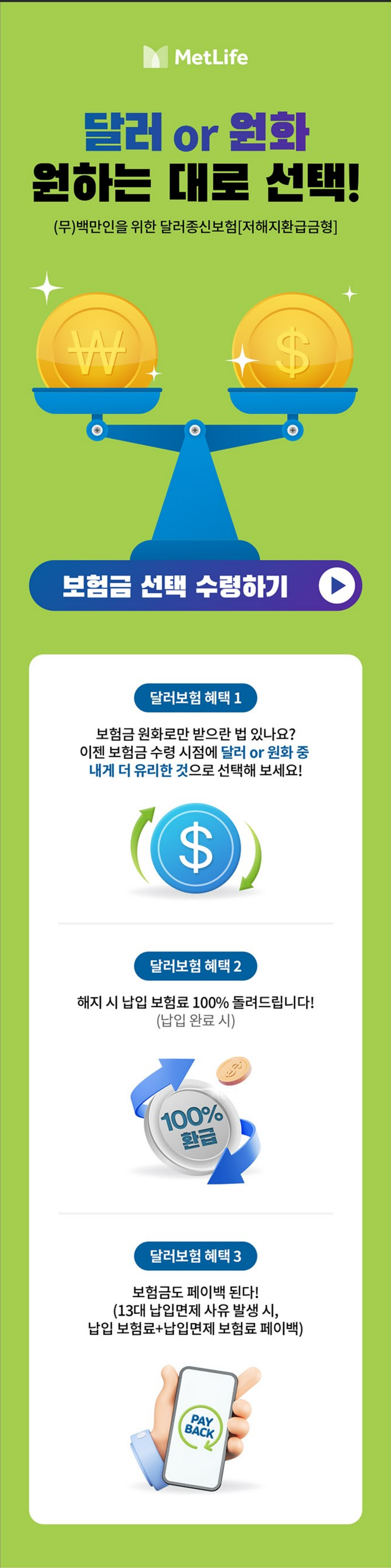
MO size (Type 1)
