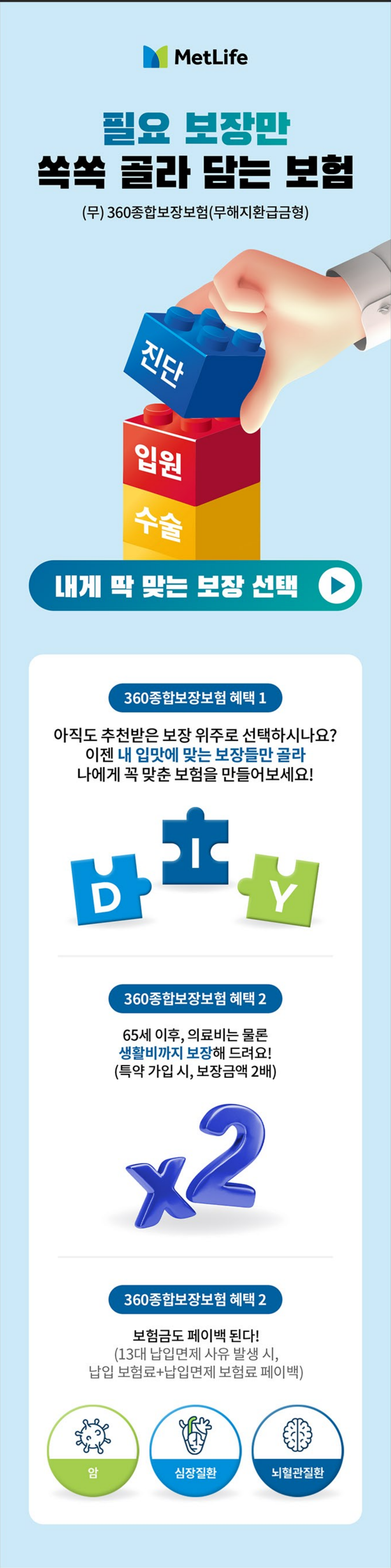
MO size (Type 2)
